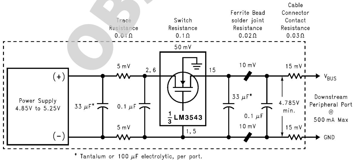
FIGURE 6. Self-Powered Hub Connections and Per-Port Voltage Drop
