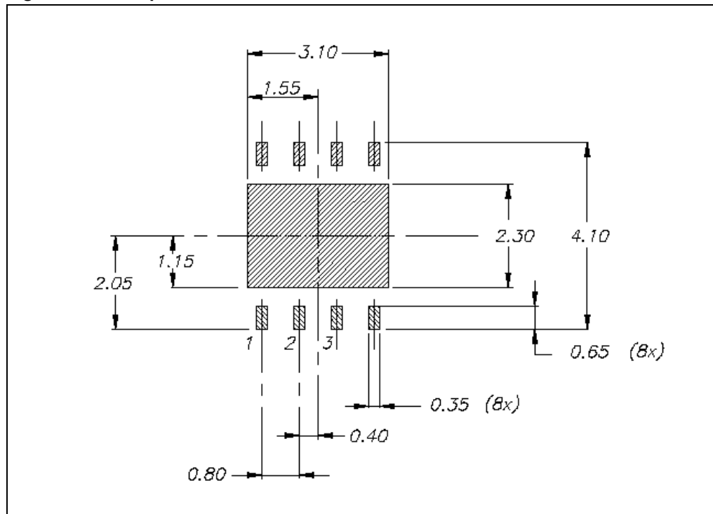
Figure 6. Foot print
