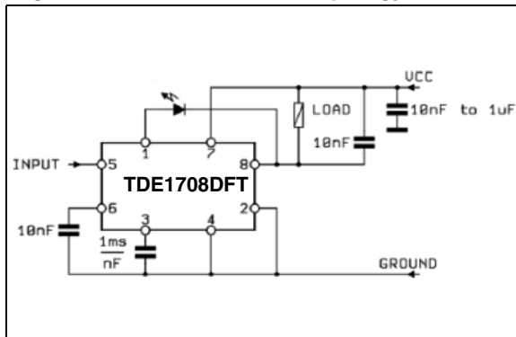
Figure 3. Low side driver topology
