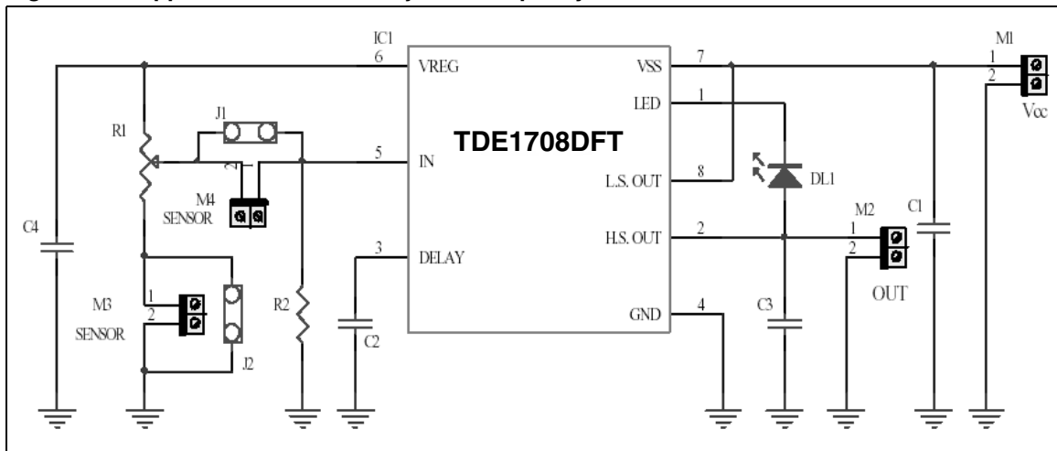
Figure 5. Application circuit for adjustable input hysteresis
