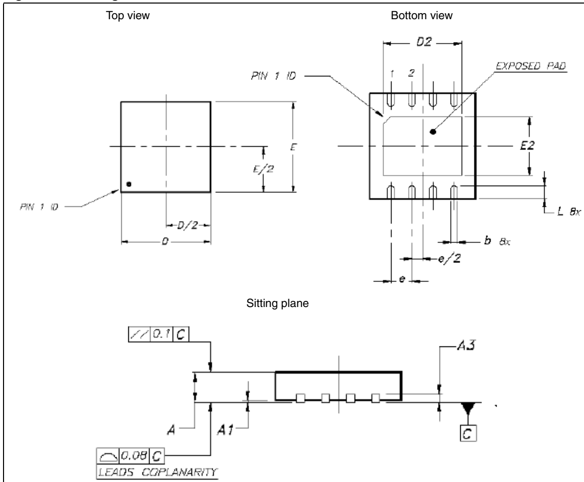
Figure 7. Package dimension
