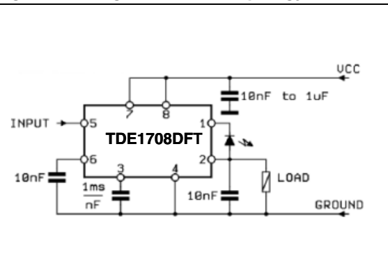
Figure 4. High side driver topology
