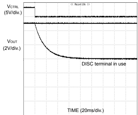
Fig.54 Discharge: CL = 47\mu F , RL = Open (BD6522F)
