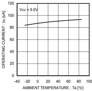
Fig.29 Operating current (CTRL enable)
