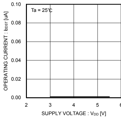
Fig.30 Operating current (CTRL disable)
