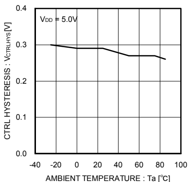
Fig.35 CTRL hysteresis voltage
