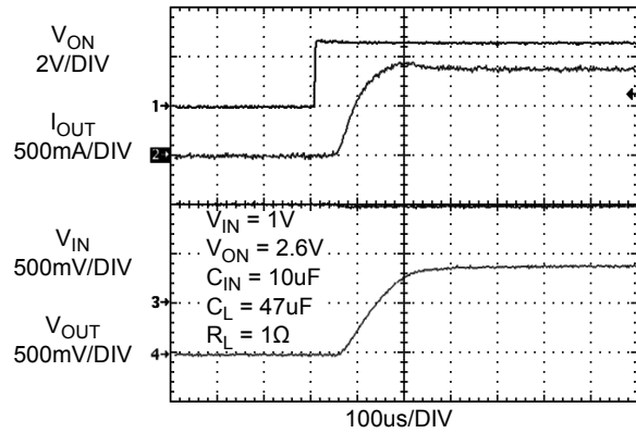
Figure 14. FPF1017 / 18 Turn On response
