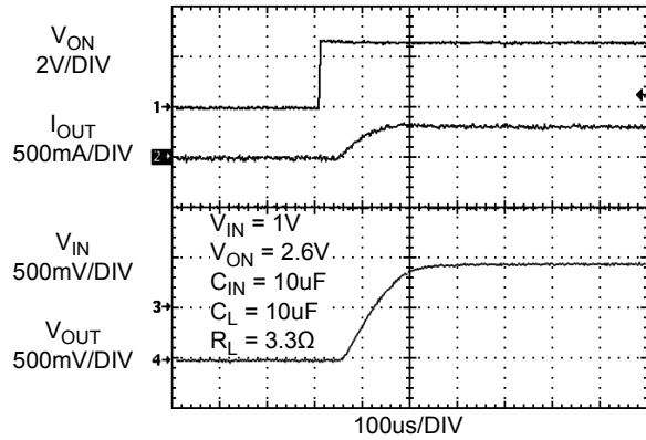
Figure 13. FPF1017 / 18 Turn On response
