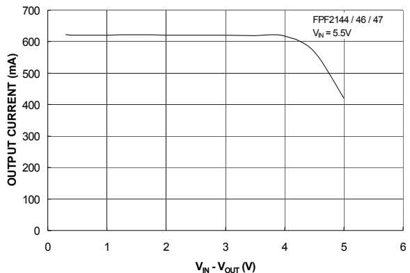
Figure 8. Current
