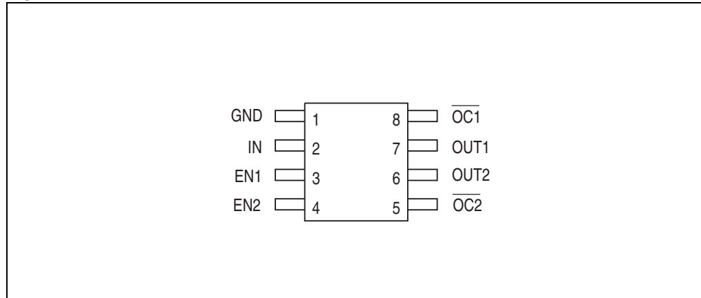
Figure 2. Pinout
