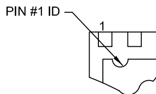
OPTIONS OF PIN ONE IDENTIFIERS
