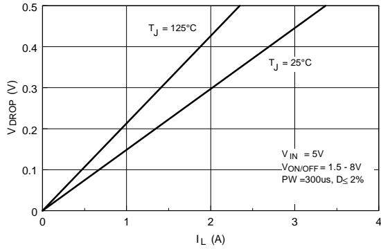
Figure 1. V_{DROP} Versus I_L at V_{IN} = 5V .
