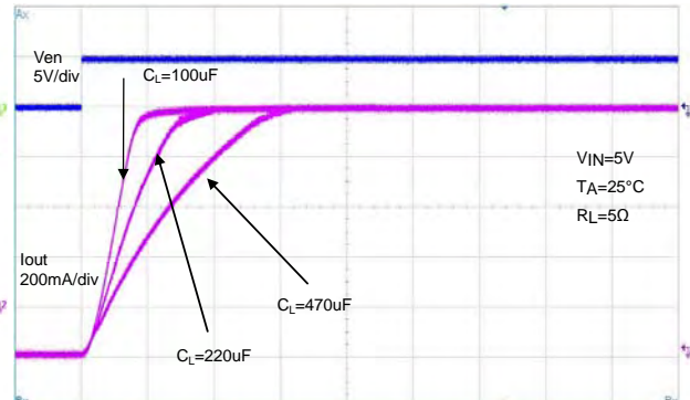
Inrush Current
