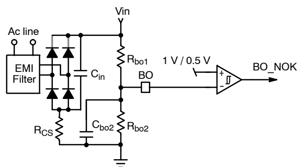
Figure 68. Brown-Out Block
