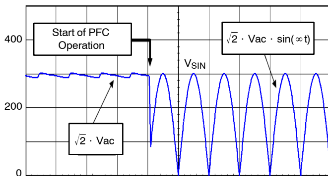
Figure 69. Typical Input Voltage of a PFC Stage
