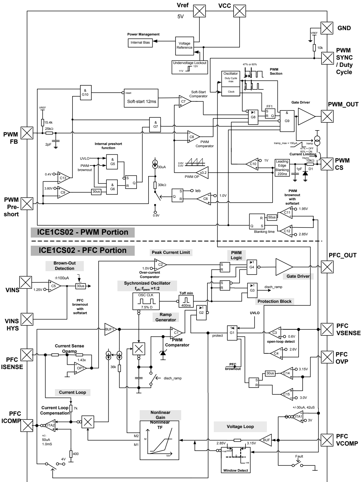
Figure 2 Representative Blockdiagram
