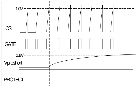
Figure 26 Pre-short Protection
