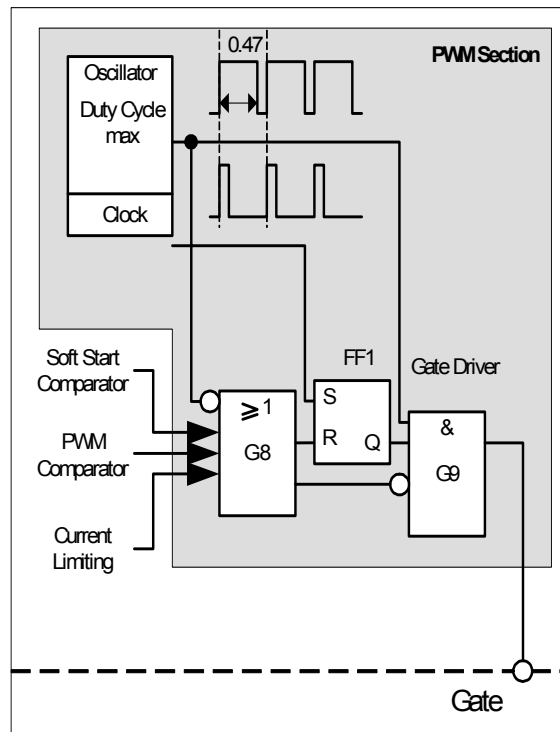
Figure 21 PWM Section
