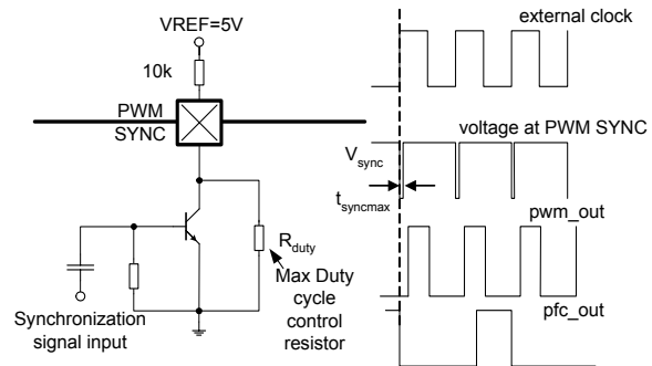
Figure 27 External Synchronization and Max Duty Selection
