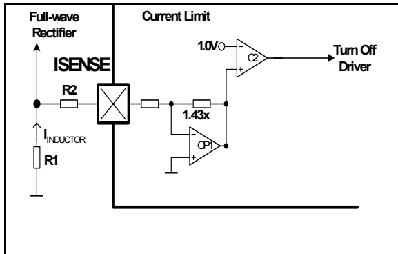
Figure 11 Peak Current Limit (PCL)
