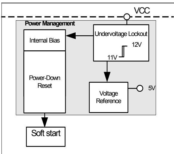
Figure 3 Power Management
