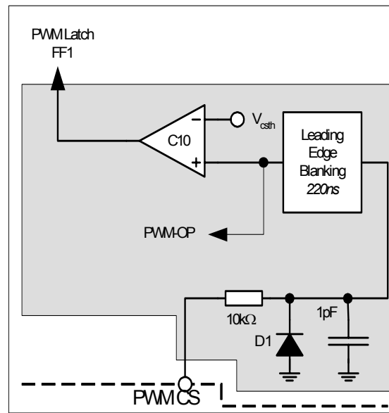
Figure 24 Current Limiting
