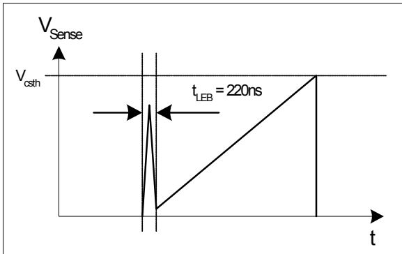
Figure 25 Leading Edge Blanking
