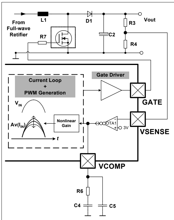
Figure 16 Voltage Loop
