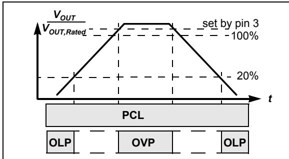
Figure 8 V_{OUT} Related Protection Features
