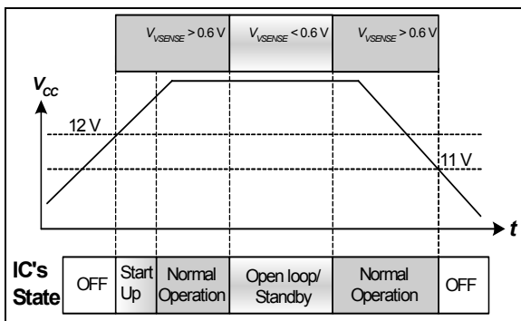
Figure 5 State of Operation respect to VCC
