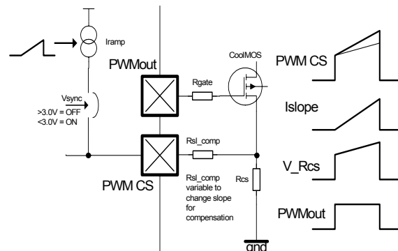
Figure 29 PWM slope compensation
