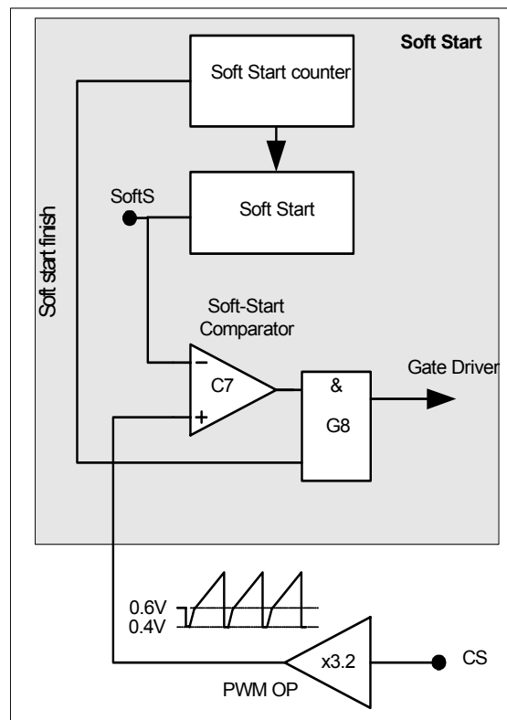
Figure 18 Soft Start
