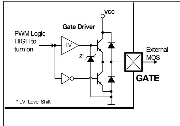
Figure 23 Gate Driver
