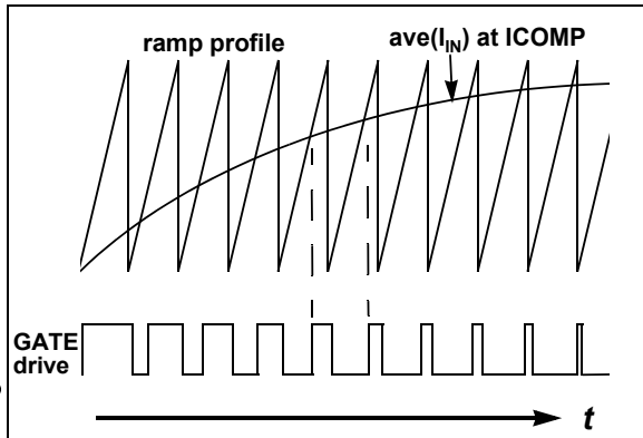
Figure 13 Average Current Control in CCM
