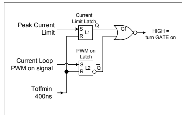
Figure 15 PWM Logic
