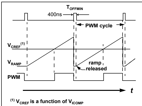
Figure 14 Ramp and PWM waveforms
