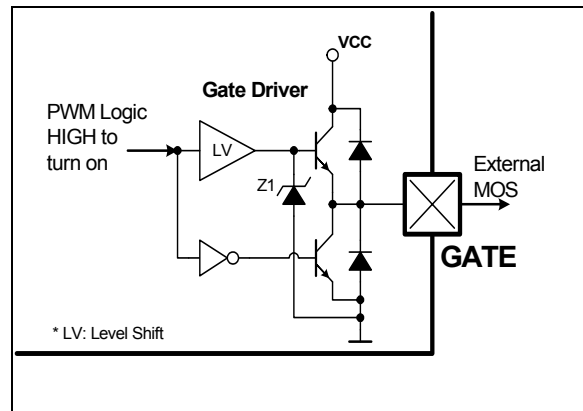
Figure 17 Gate Driver
