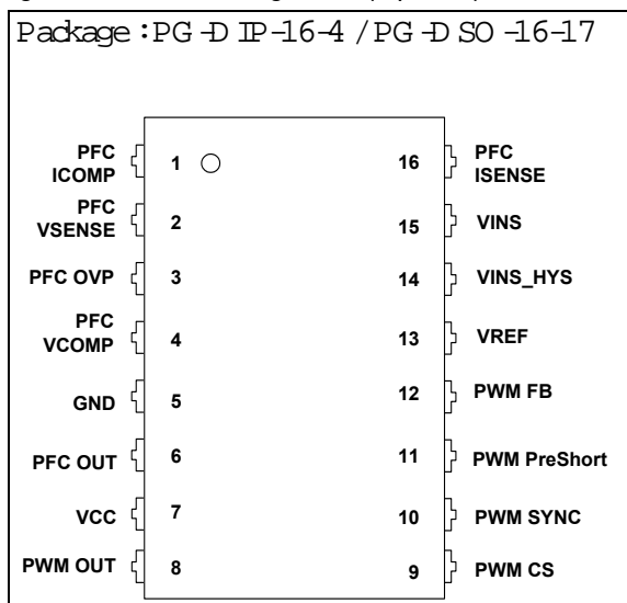
Figure 1 Pin Configuration (top view)
