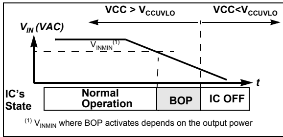
Figure 7 V_{IN} Related Protection Features
