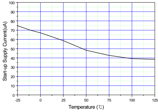
Figure 7. Start-Up Supply Current vs Temperature
