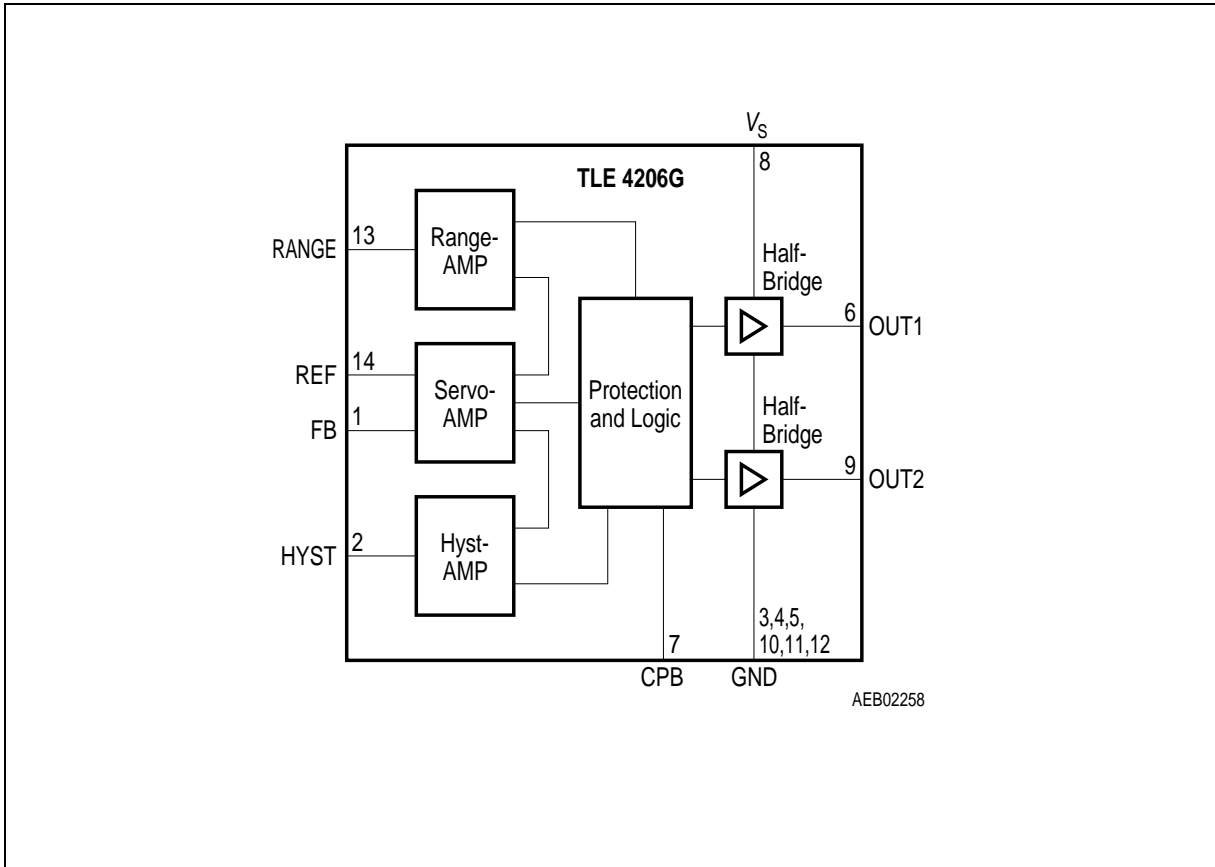
Figure 2 Block Diagram (Pin numbers are valid for TLE 4206 G in P-DSO-14-8)
