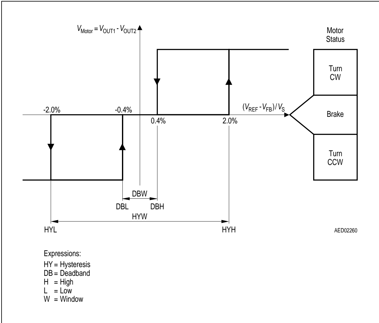
Figure 4 Hysteresis, Phaselag and Deadband-Definitions
