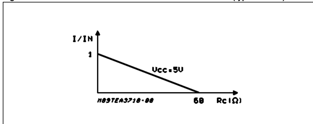
Figure 18. Current reduction in the motor on alarm condition (typical curve)
