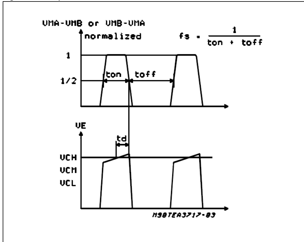
Figure 7. Output waveforms
