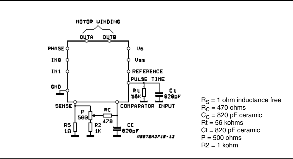
Figure 6. Typical external component configuration
