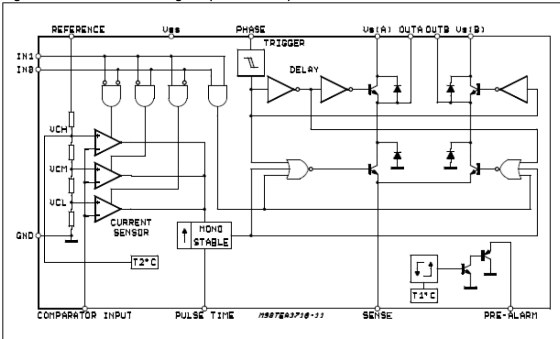
Figure 4. Detailed block diagram (TEA3718SP)
