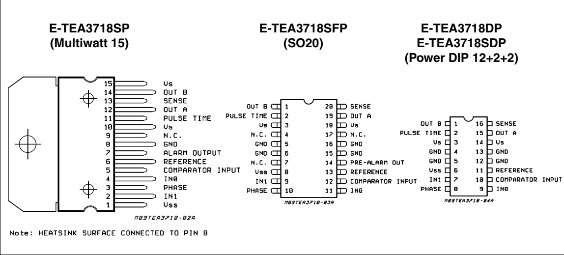
Figure 2. Package pin locations (top views)
