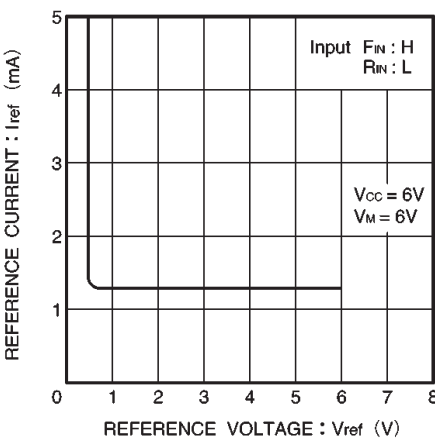
Fig.11 V_{REF} reference current vs. V_{REF} reference voltage
