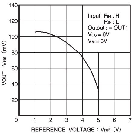
Fig.10 V_{OUT} - V_{REF} voltage differential vs. V_{REF} reference voltage
