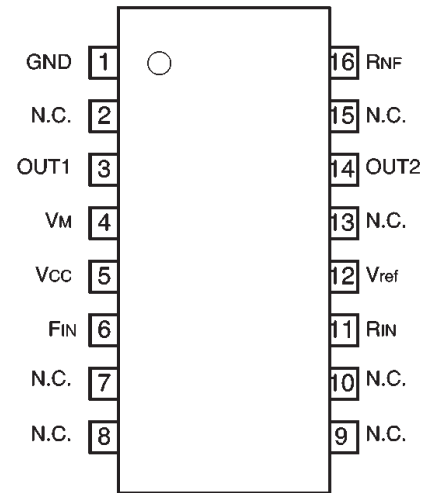
Fig.1 Pin assignments
