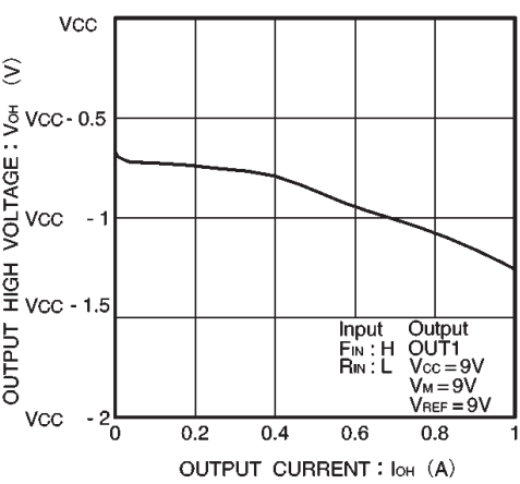
Fig.8 Output high level voltage vs. output current
