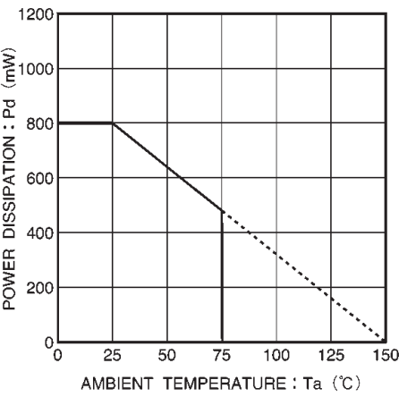
Fig.6 Power dissipation curve
