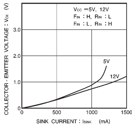
Fig.8 Output saturated voltage vs. sink current ( I )
