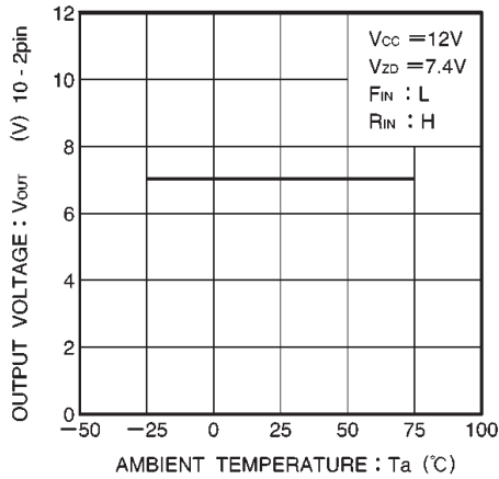
Fig.7 Output voltage vs. ambient temperature
