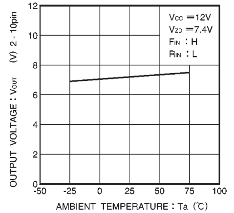
Fig.6 Output voltage vs. ambient temperature
