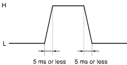
Fig.17 Control signal
