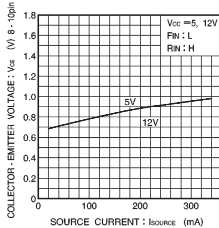
Fig.11 Output saturated voltage vs. source current ( II )
