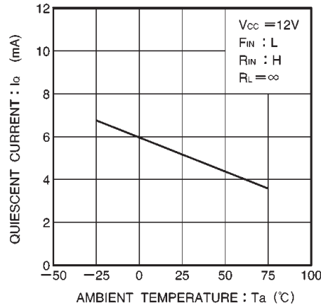
Fig.5 Quiescent current vs. ambient temperature
