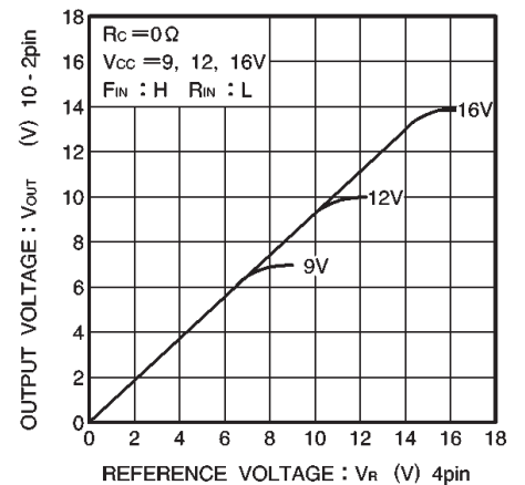
Fig.12 Output voltage vs. reference voltage ( I )
