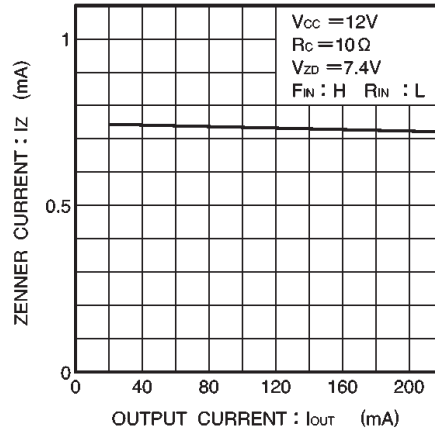
Fig.14 Zener current vs. output current
