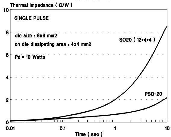
Figure 12. Thermal Impedance of PowerSO-20 and standard SO20
