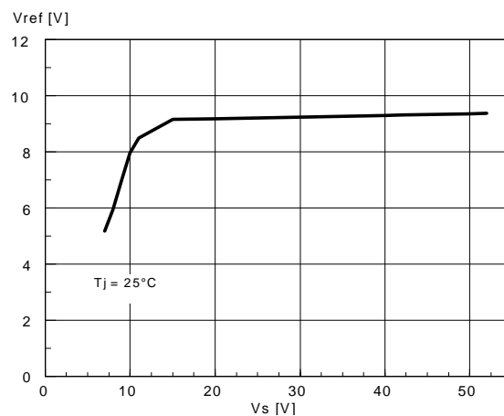
Figure 6. Reference Voltage vs. Supply Voltage.
