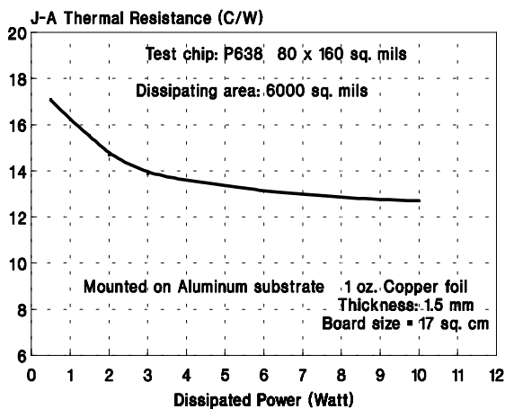
Figure 11. PowerSO-20: with external heatsink
