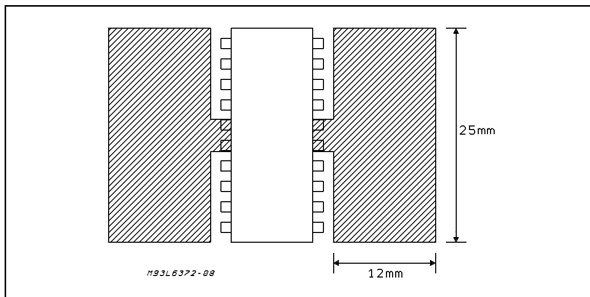
Figure 1: Printed Heatsink
