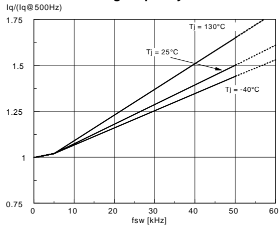
Figure 2. Normalized Quiescent Current vs. switching frequency.
