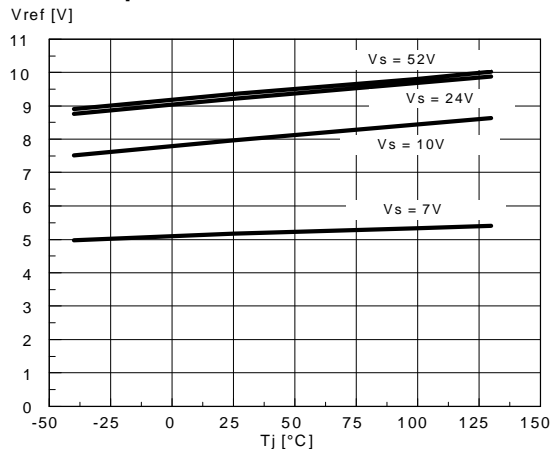
Figure 7. Reference Voltage vs. Junction Temperature.
