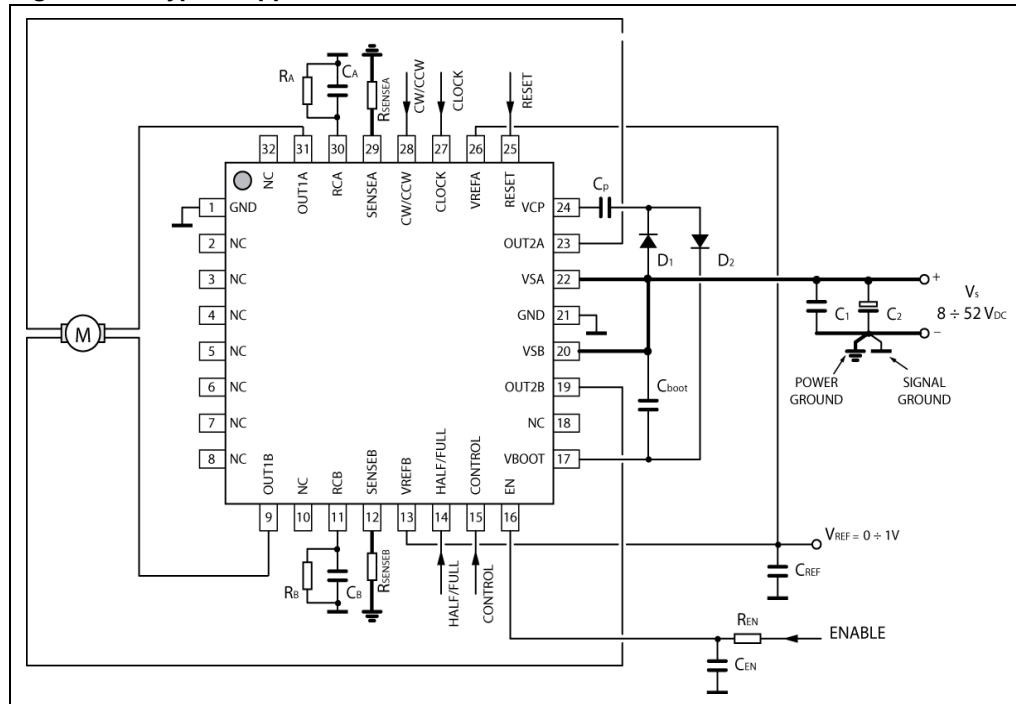
Figure 25. Typical application
