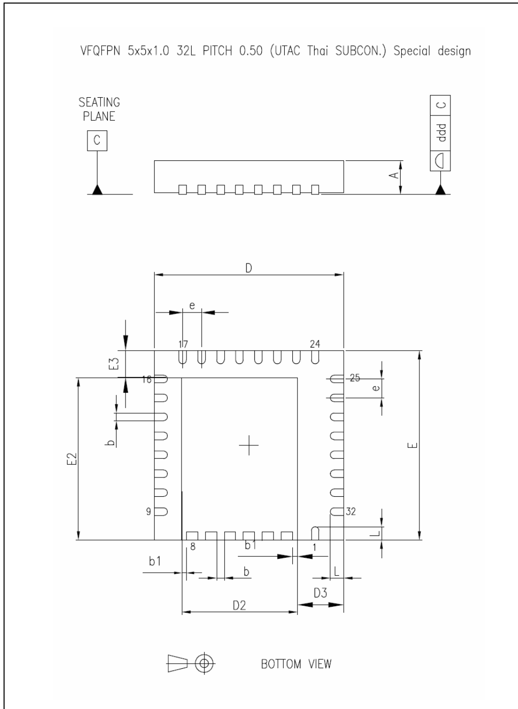
Figure 30. Package dimensions
