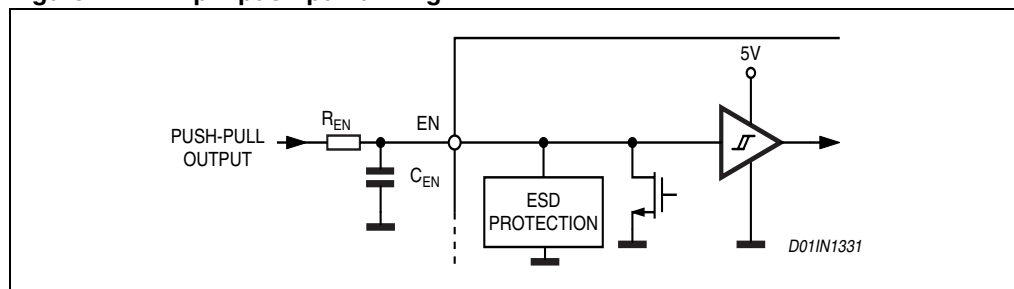
Figure 11. EN pin push-pull driving
