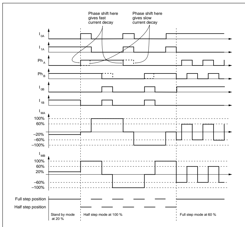
Figure 6. Principal operating sequence
