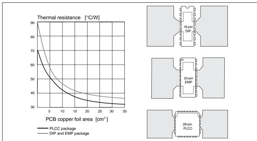
Figure 10. Copper foil used as a heatsink
