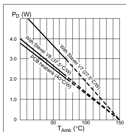
Figure 16. Allowable power dissipation vs. ambient temperature
