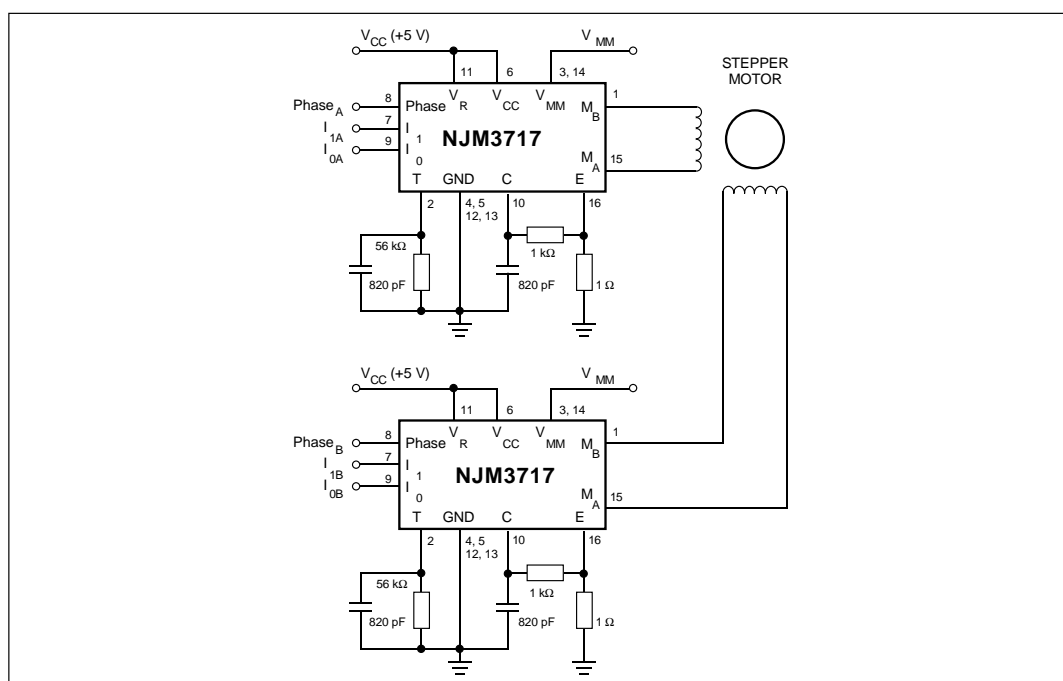
Figure 8. Typical stepper motor driver application with NJM3717
