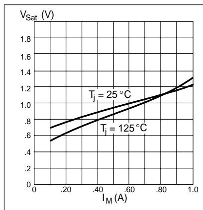
Figure 12. Typical sink saturation vs. output current
