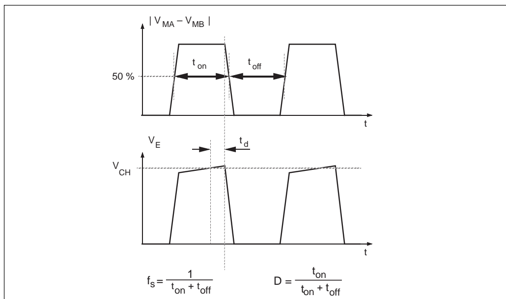
Figure 3. Definition of terms
