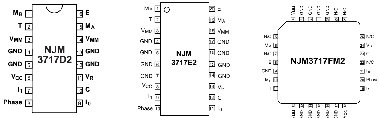
Figure 2. Pin configurations
