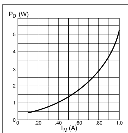
Figure 15. Typical power dissipation vs. motor current
