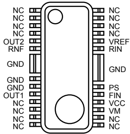
Fig.32 BA6285AFP-Y (HSOP25)
