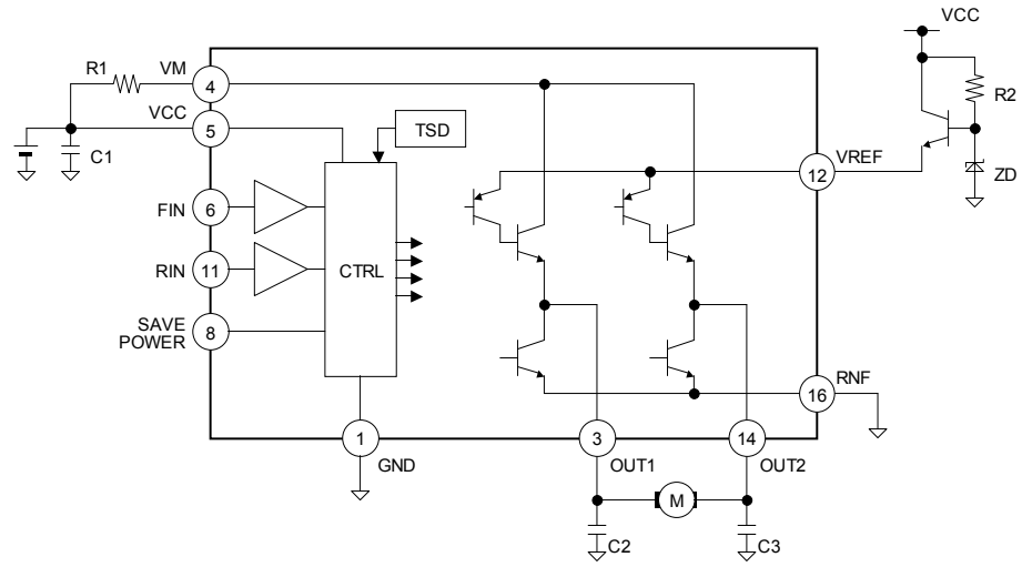
Fig.29 BA6285FS
