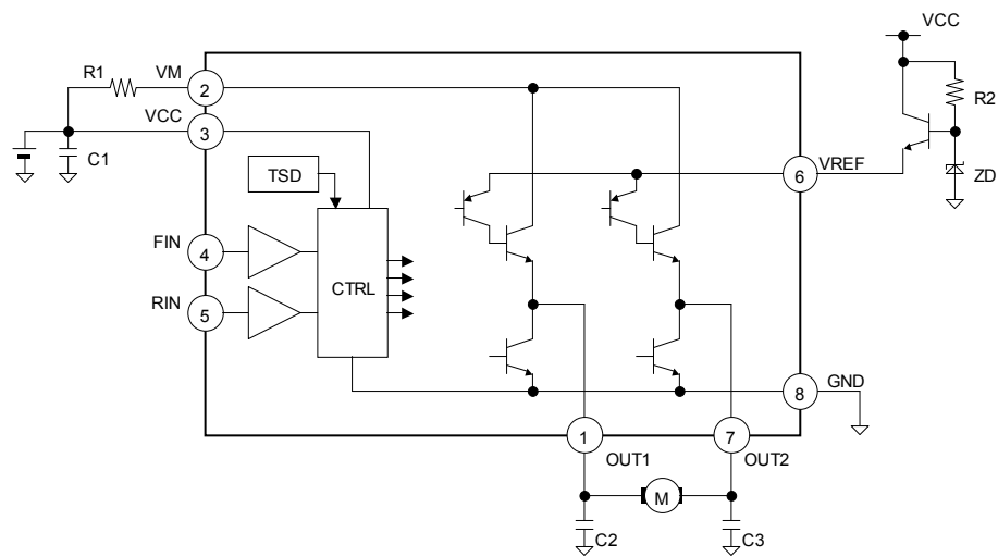
Fig.27 BA6287F
