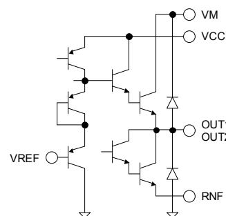
Fig.39 POWER SAVE
