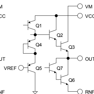
Fig.37 BA6920FP-Y
