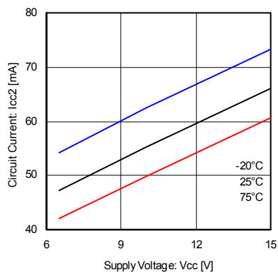
Fig.2 Supply current 2 (brake) (BA6956AN)
