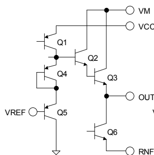
Fig.36 BA6956AN
