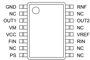
Fig.30 BA6285FS (SSOP-A16)
