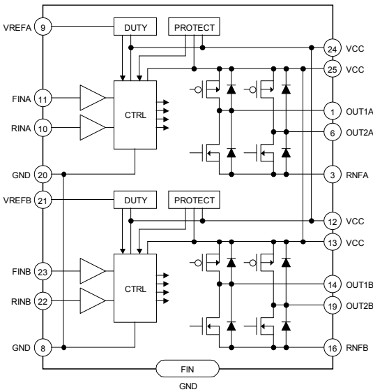
Fig.31 BD6215FP / BD6216FP
