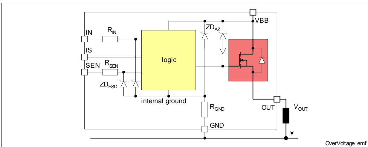
Figure 12 Over-Voltage Protection
