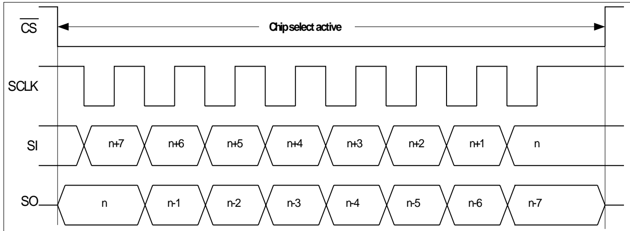
Figure 11 Serial interface
