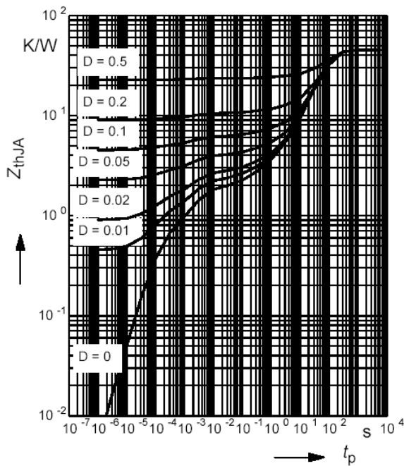
Typ. transient thermal impedance Z_{\text{thJA}}=f(t_p) @ min. footprint
