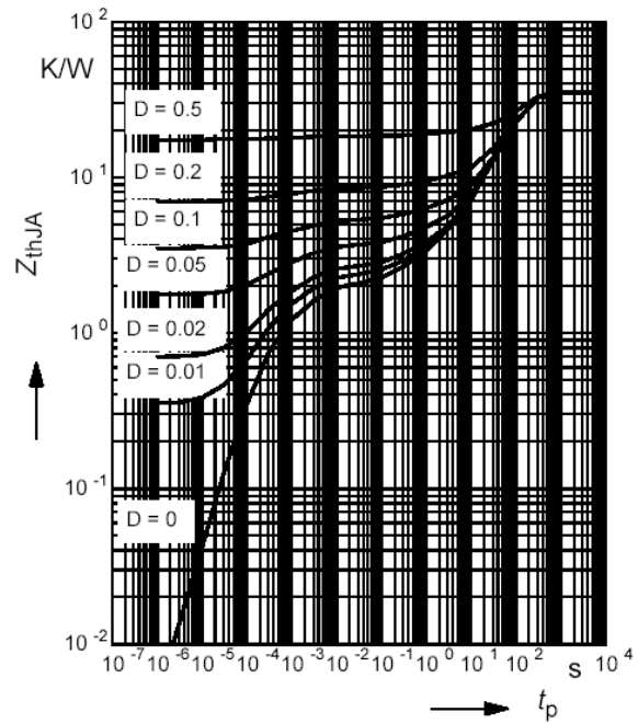
Typ. transient thermal impedance Z_{\text{thJA}}=f(t_p) @ 6cm² heatsink area
