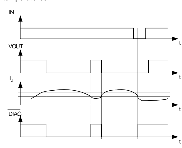
Figure 5 Overtemperature detection
