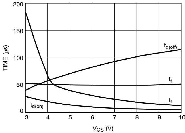
Figure 16. Resistive Load Switching Time vs. Gate-Source Voltage ( V_{DD} = 25 \text{ V} , I_D = 5 \text{ A} , R_G = 0 \Omega )
