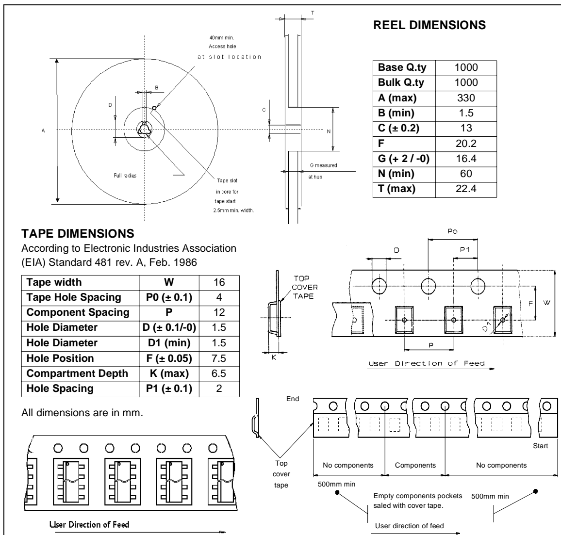
Figure 48. Tape And Reel Shipment (Suffix "TR")
