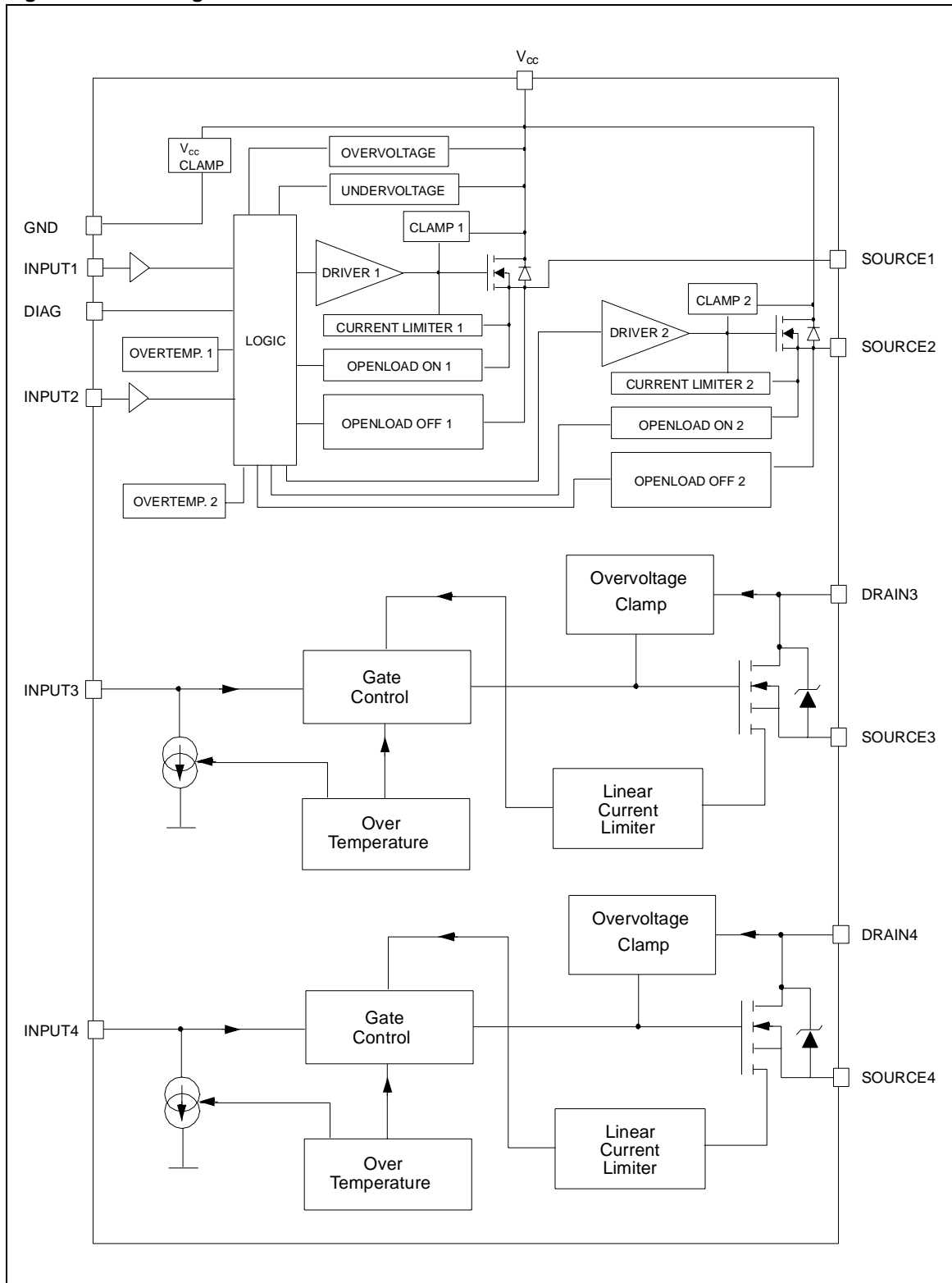
Figure 2. Block Diagram
