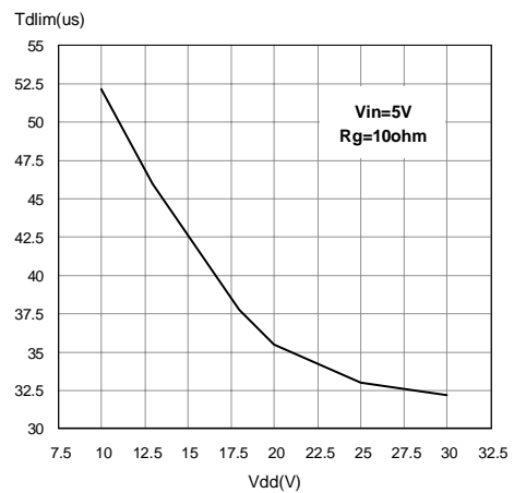
Figure 36. Step Response Current Limit
