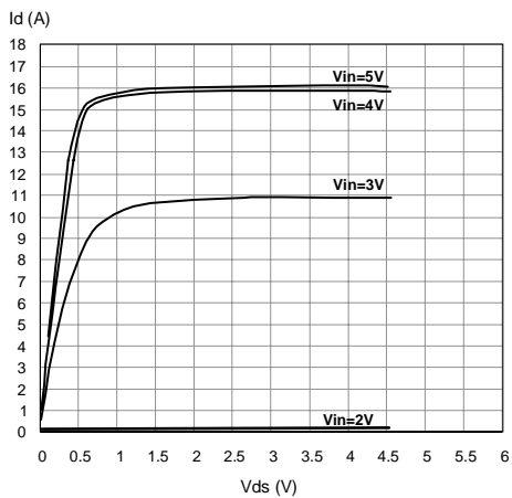
Figure 33. Output Characteristics
