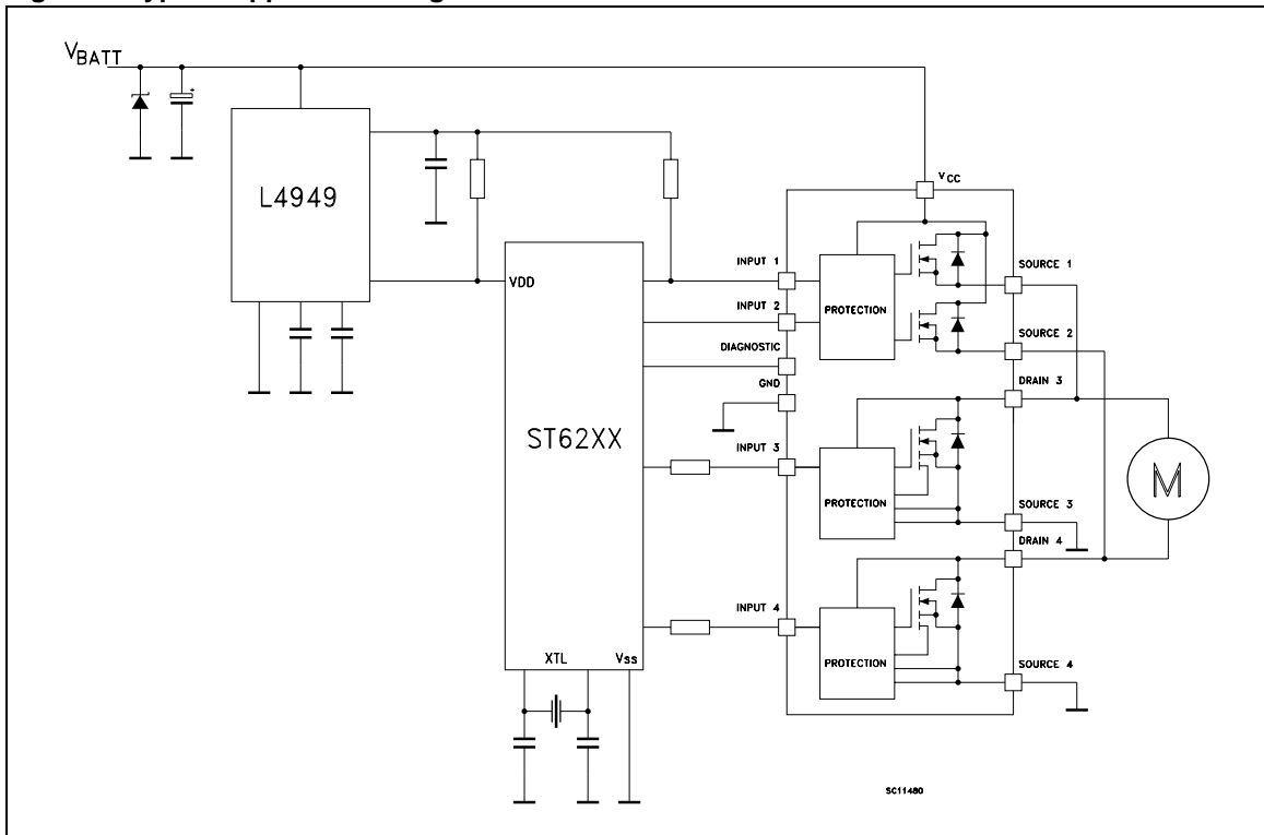
Figure 6. Typical Application Diagram
