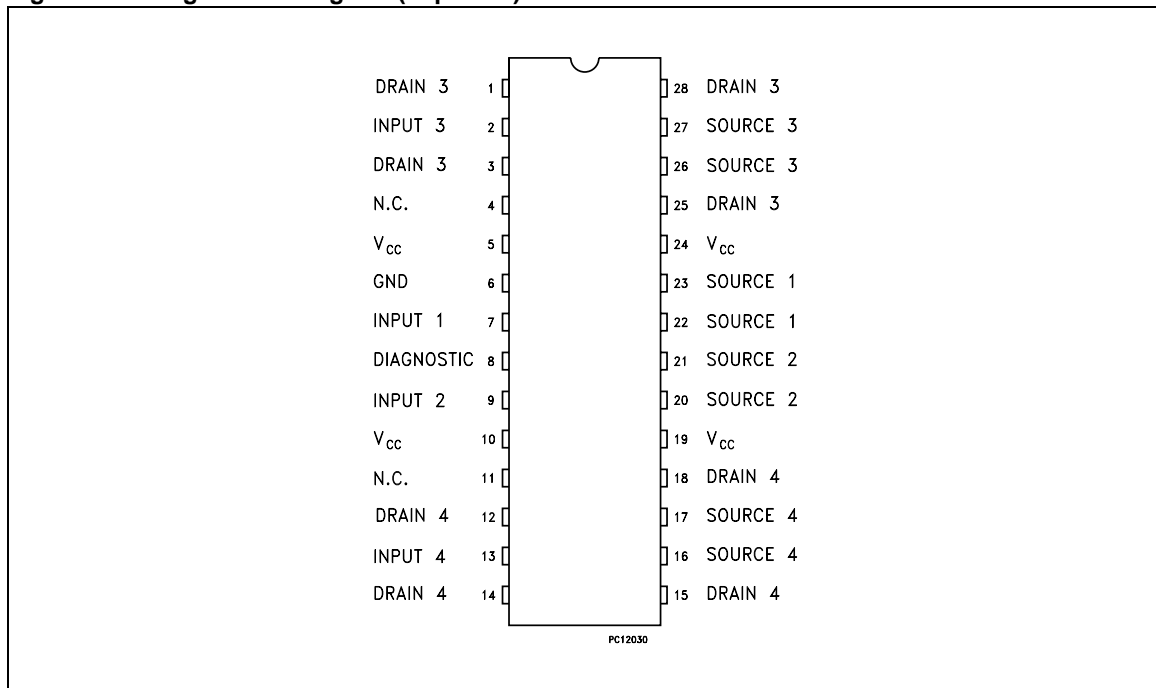
Figure 3. Configuration Diagram (Top View)
