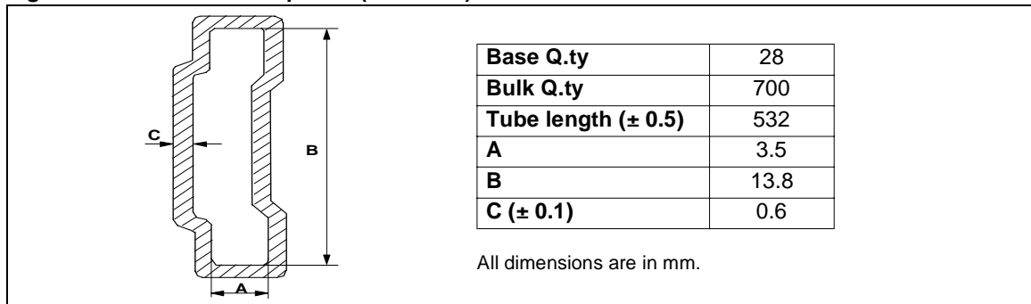
Figure 47. SO-28 Tube Shipment (No Suffix)
