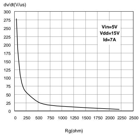
Figure 45. Turn off drain source voltage slope
