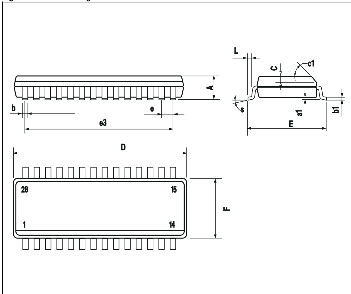
Figure 46. SO-28 Package Dimensions
