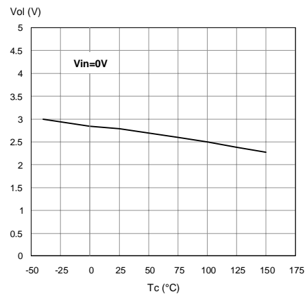
Figure 24. Openload Off State Voltage Detection Threshold
