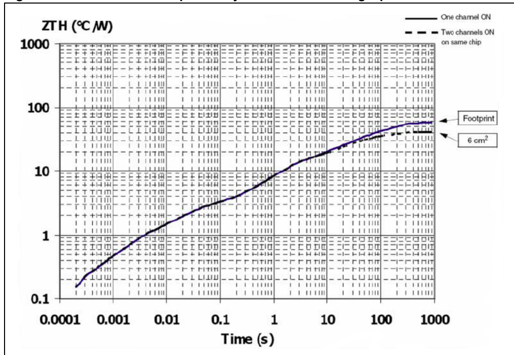
Figure 30. SP-28 thermal impedance junction ambient single pulse
