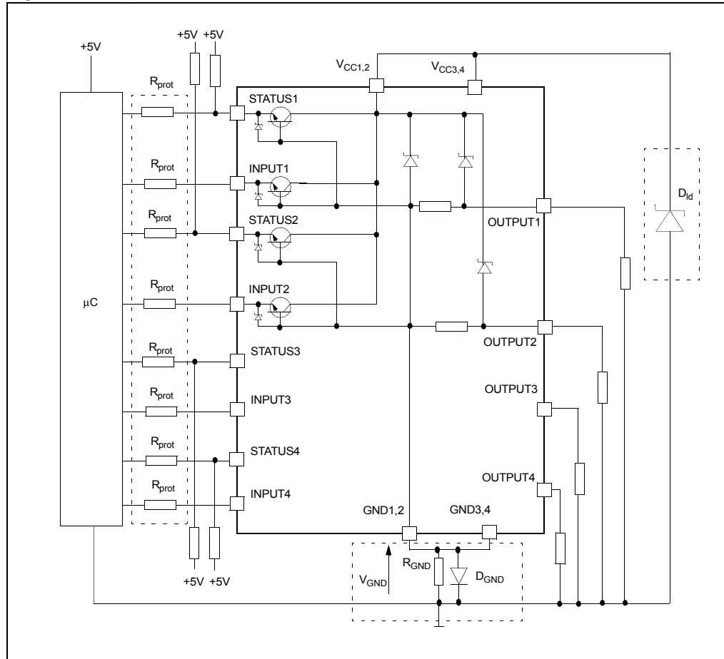
Figure 25. Application schematic
