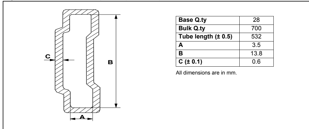
Figure 33. SO-28 tube shipment (no suffix)
