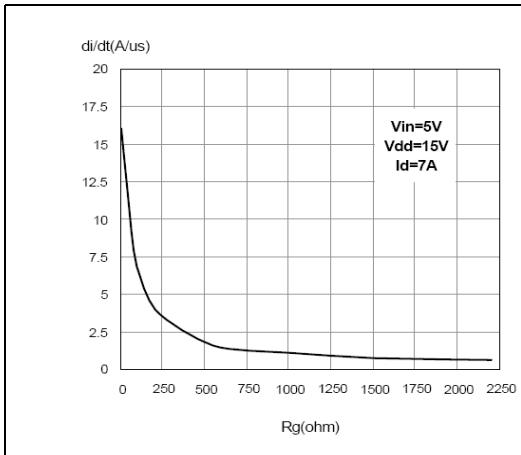
Figure 27. Turn-on current slope (Vin=5V)
