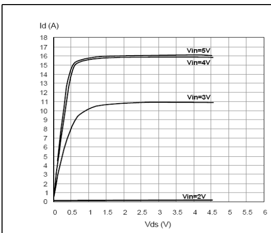
Figure 33. Output characteristics
