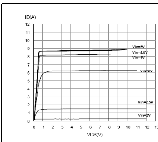
Figure 33. Output characteristics
