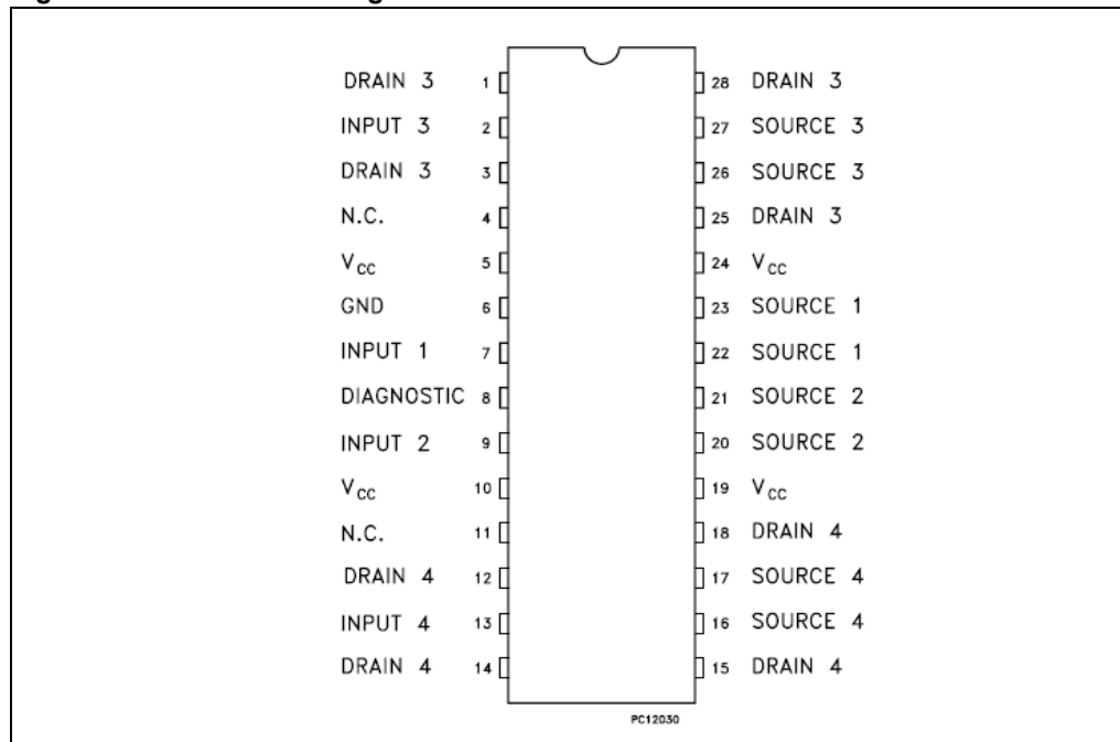
Figure 2. Connection diagram
