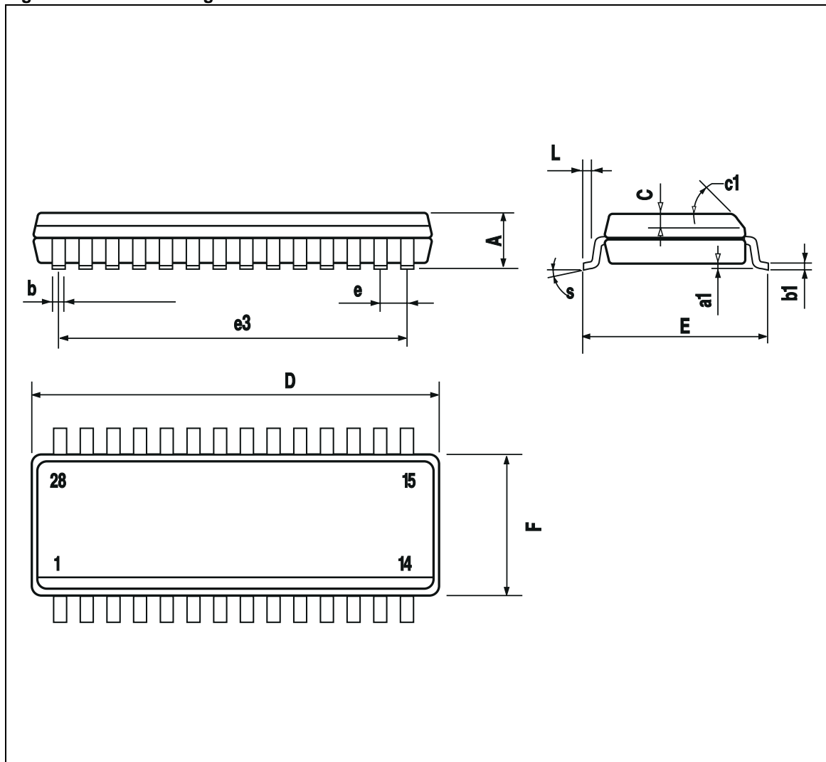
Figure 46. SO-28 Package Dimensions
