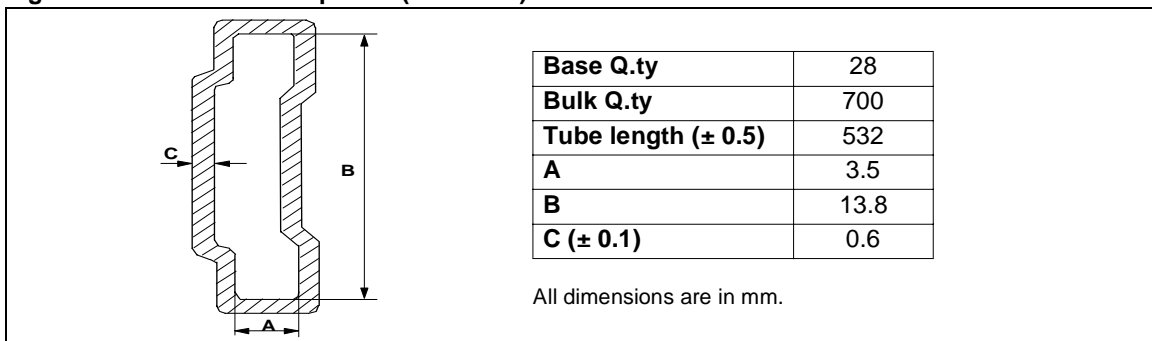
Figure 47. SO-28 Tube Shipment (No Suffix)
