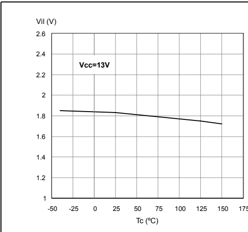
Figure 11. Input low level
