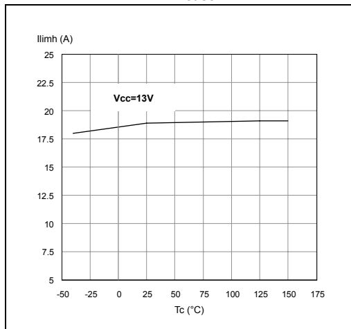
Figure 20. I_{LIMH} vs T_{case}
