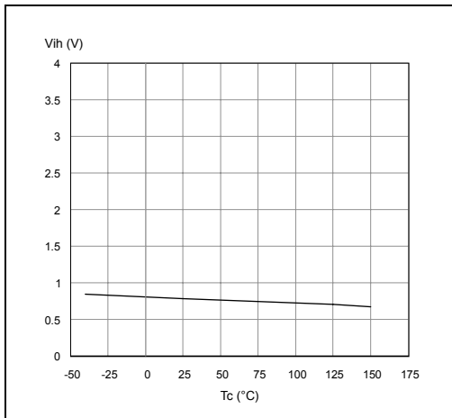
Figure 14. Input high level
