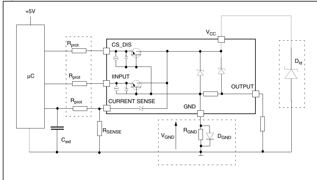
Figure 25. Application schematic
