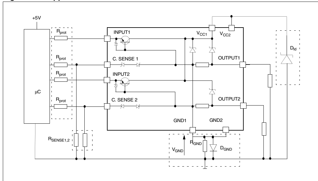
Figure 19. Application schematic
