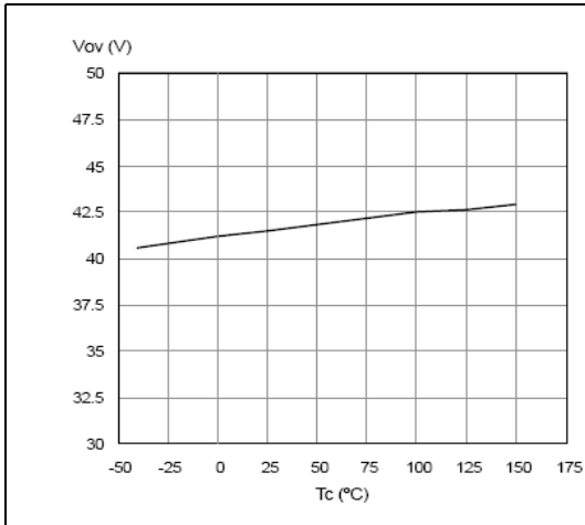
Figure 14. Turn-on voltage slope
