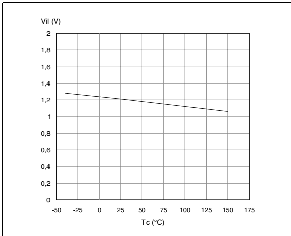
Figure 19. Input low level
