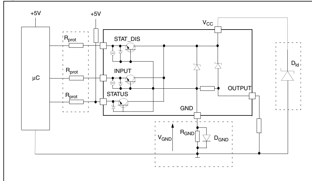
Figure 32. Application schematic
