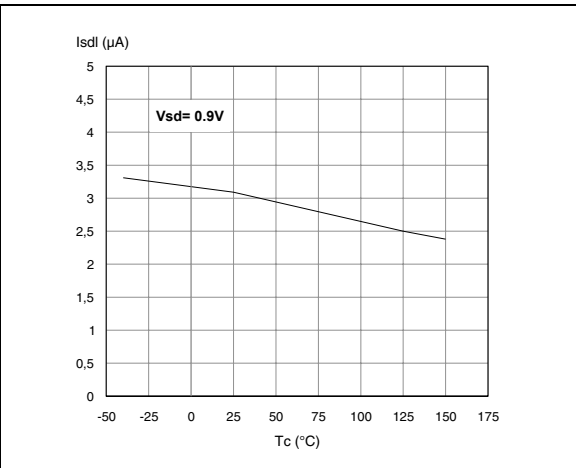
Figure 20. Low level STAT_DIS current
