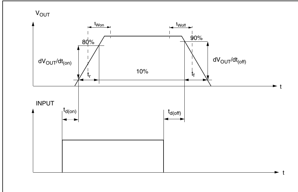
Figure 6. Switching characteristics
