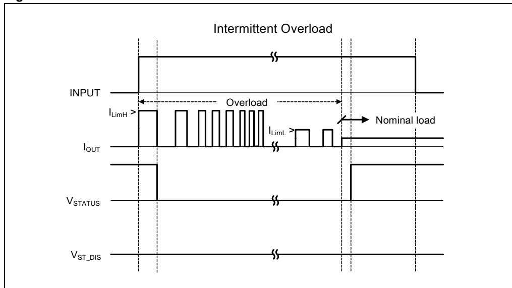
Figure 10. Intermittent Overload
