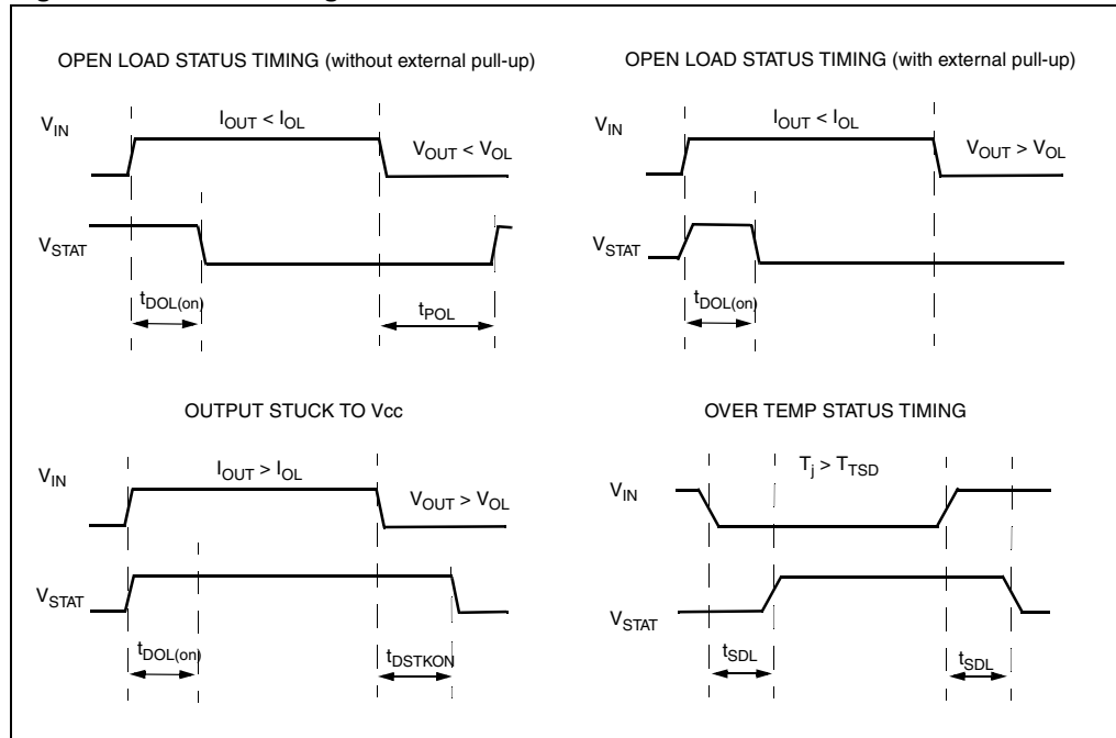
Figure 4. Status timings
