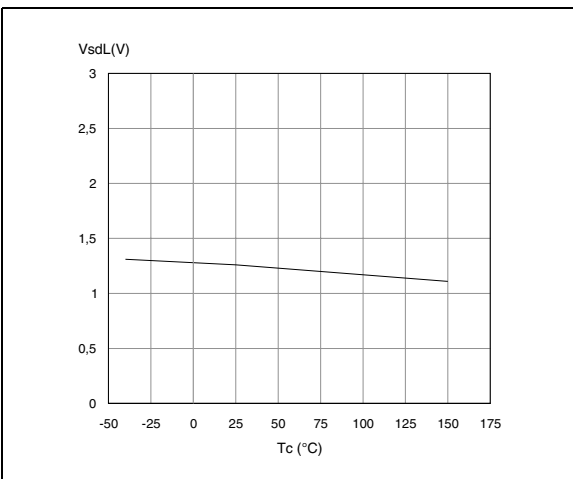
Figure 31. Low level STAT_DIS voltage
