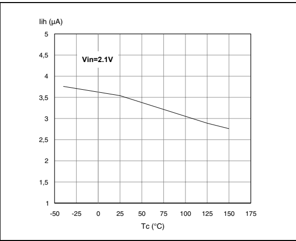
Figure 18. Input high level
