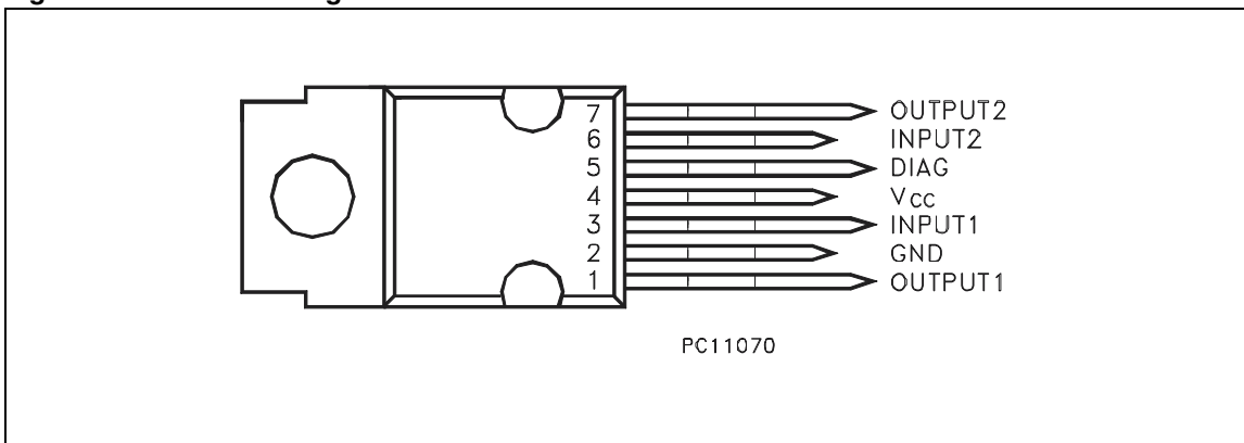
Figure 3. Connection Diagram
