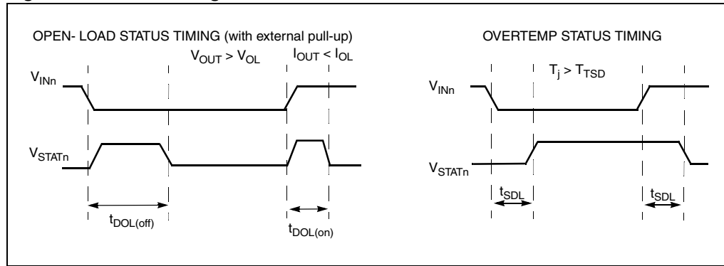
Figure 4. Status timings
