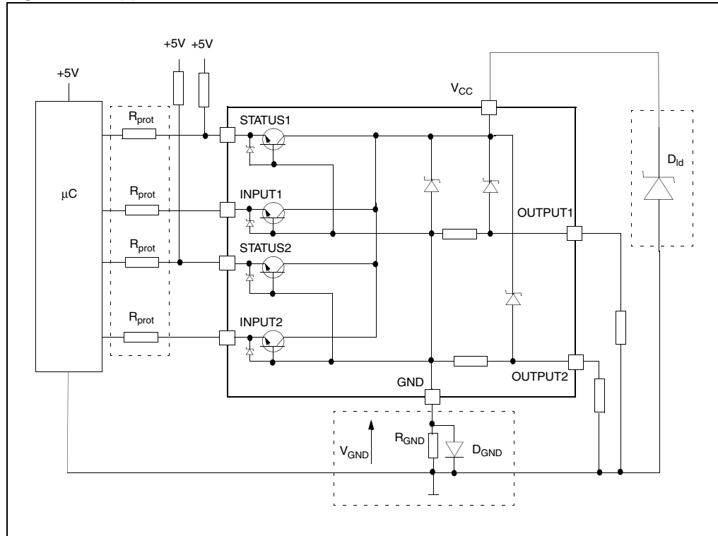
Figure 25. Application schematic
