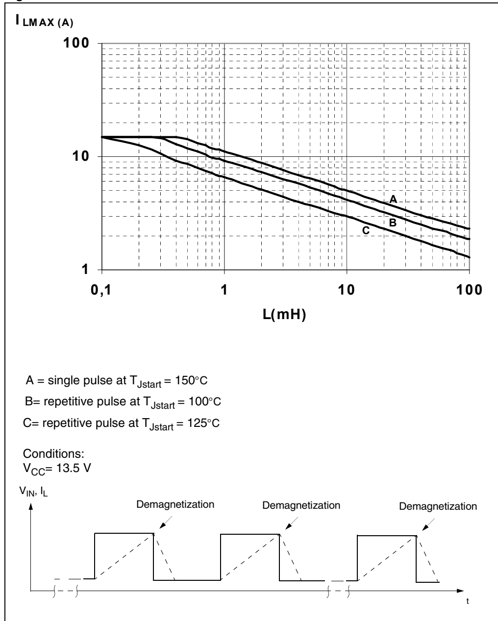
Figure 27. Maximum turn-off current versus load inductance
