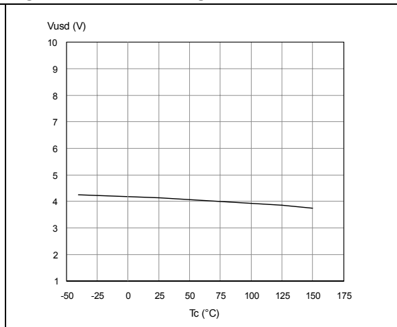
Figure 24. Undervoltage shutdown
