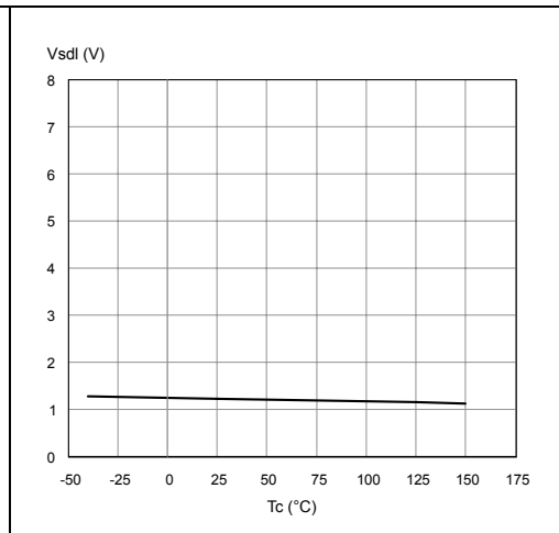
Figure 26. Low level STAT_DIS voltage
