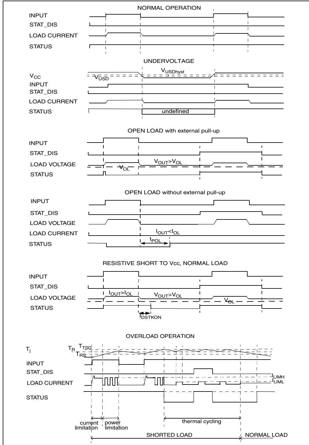
Figure 29. Waveforms
