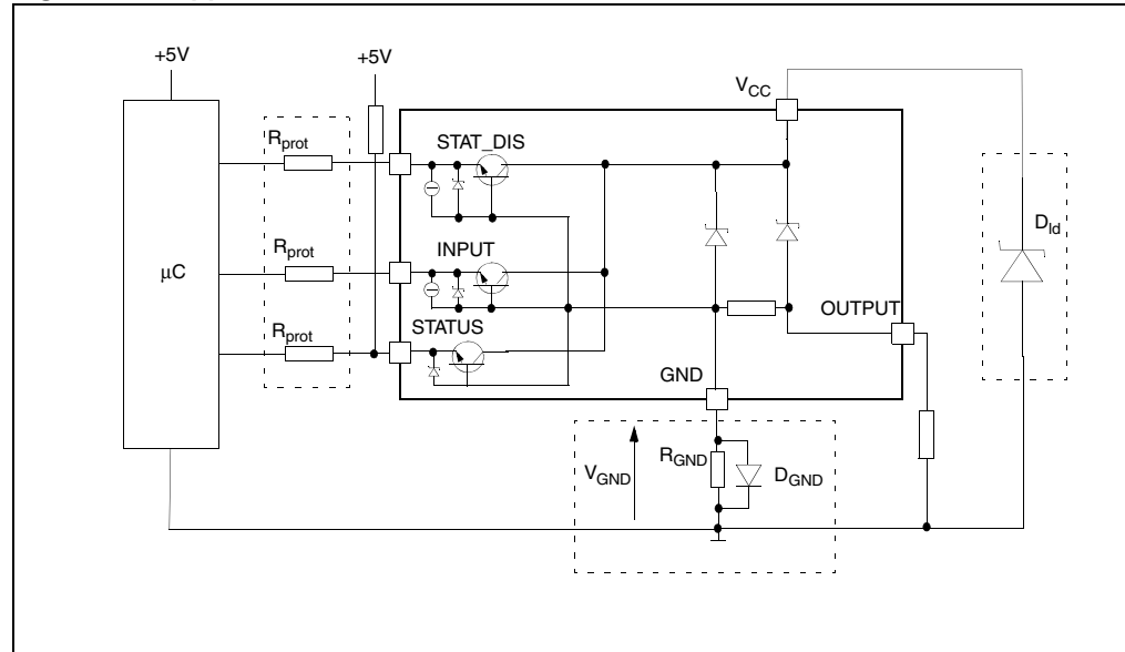
Figure 27. Application schematic
