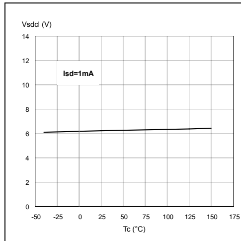
Figure 25. STAT_DIS clamp voltage
