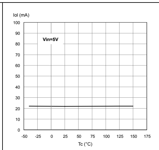
Figure 18. Open-load on-state detection threshold
