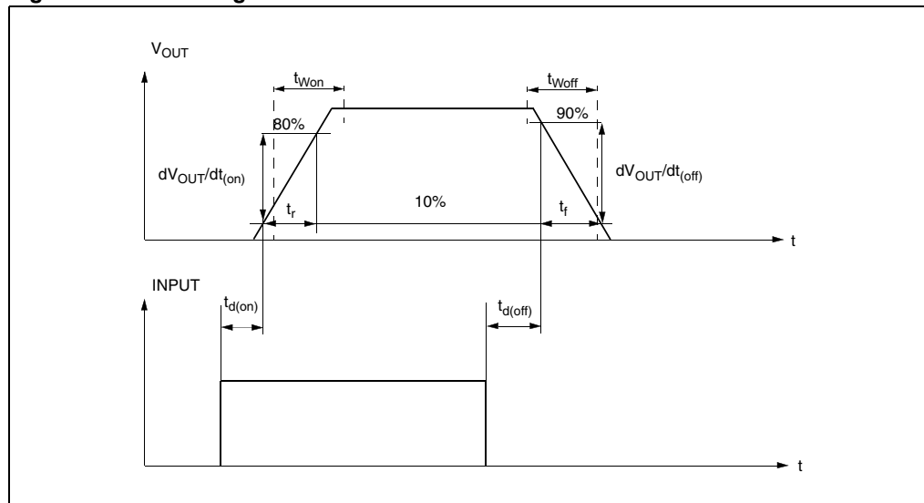
Figure 6. Switching characteristics
