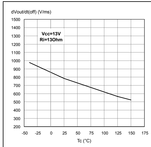
Figure 23. Turn-off voltage slope
