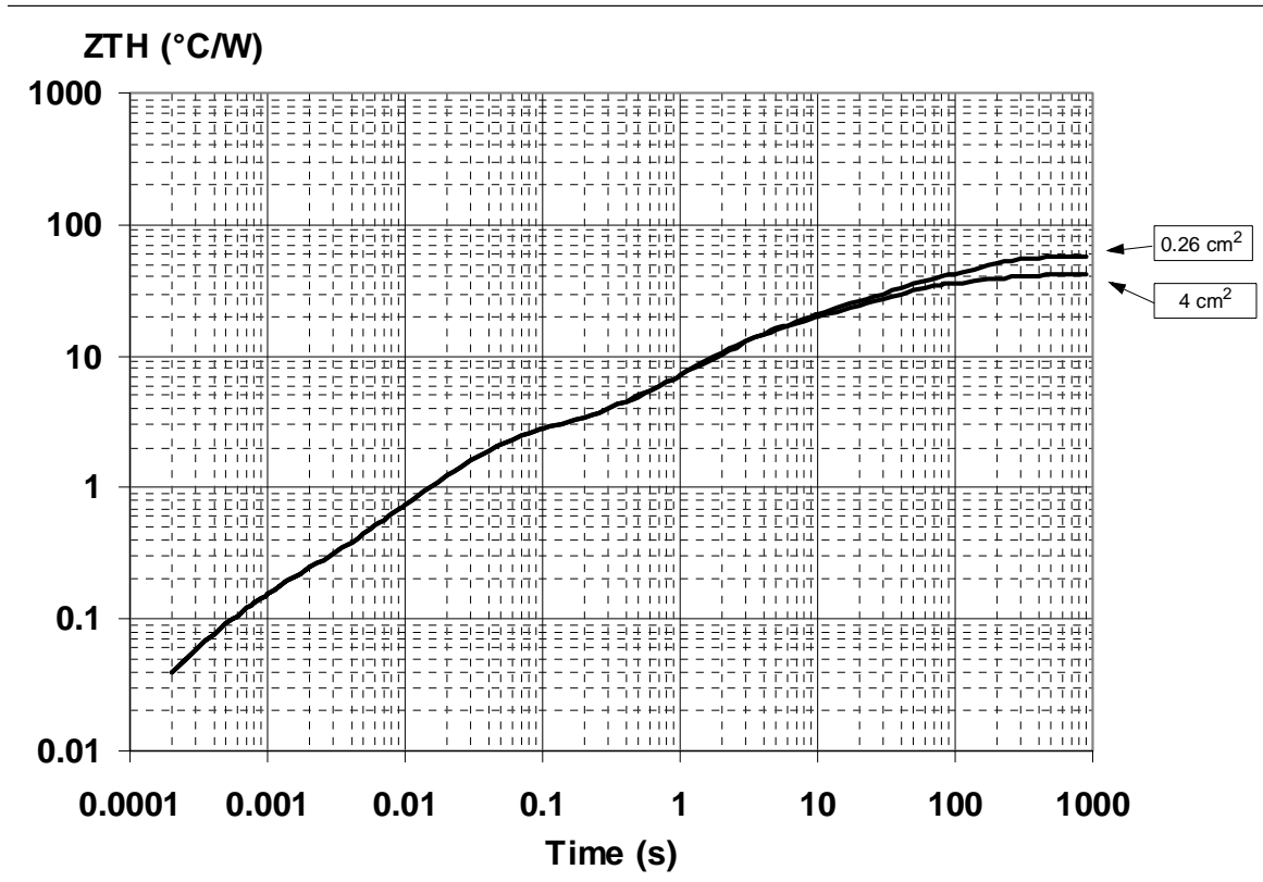
Figure 30. SO-16 Thermal Impedance Junction Ambient Single Pulse
