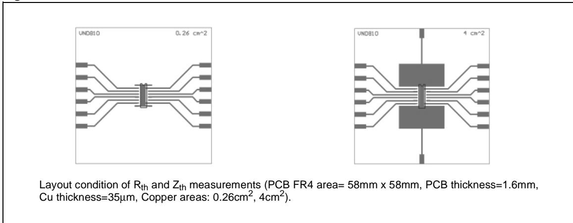
Figure 28. SO-16 PC Board
