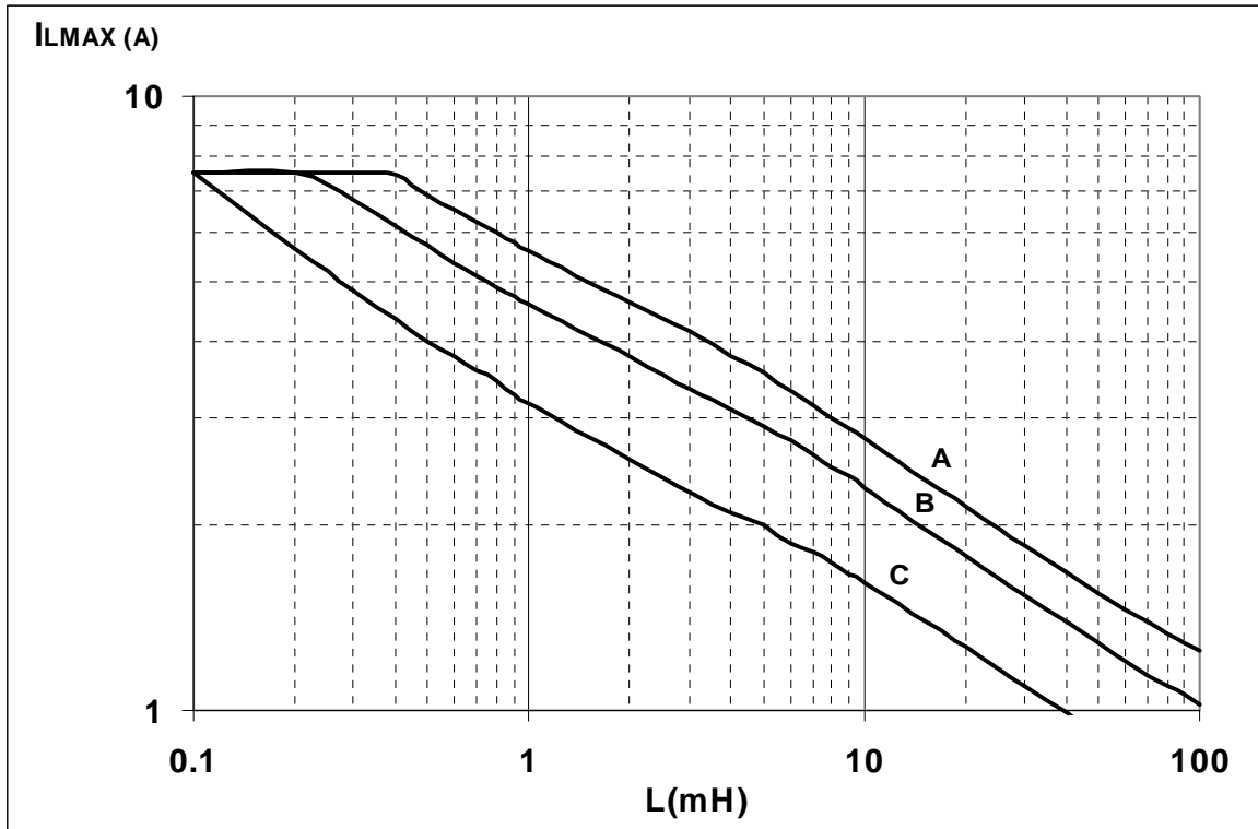
Figure 27. Maximum turn off current versus load inductance
