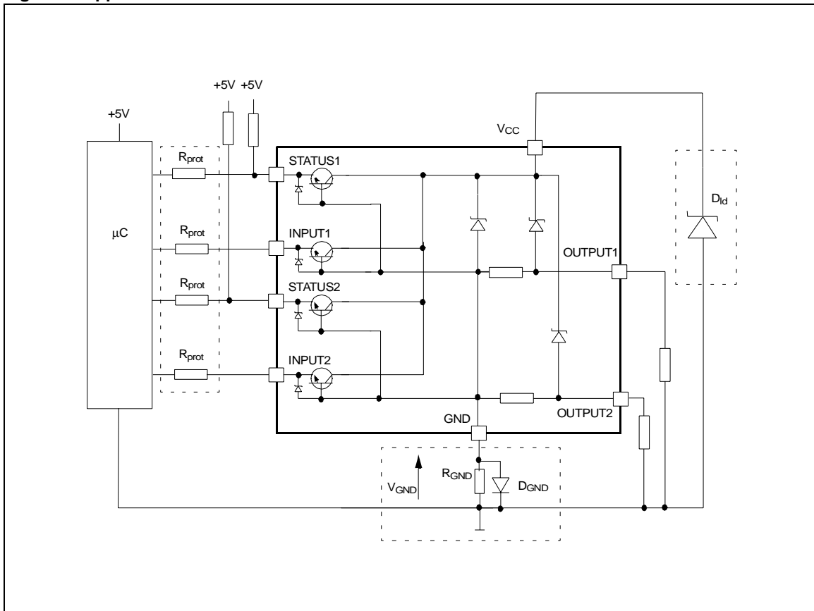
Figure 8. Application Schematic
