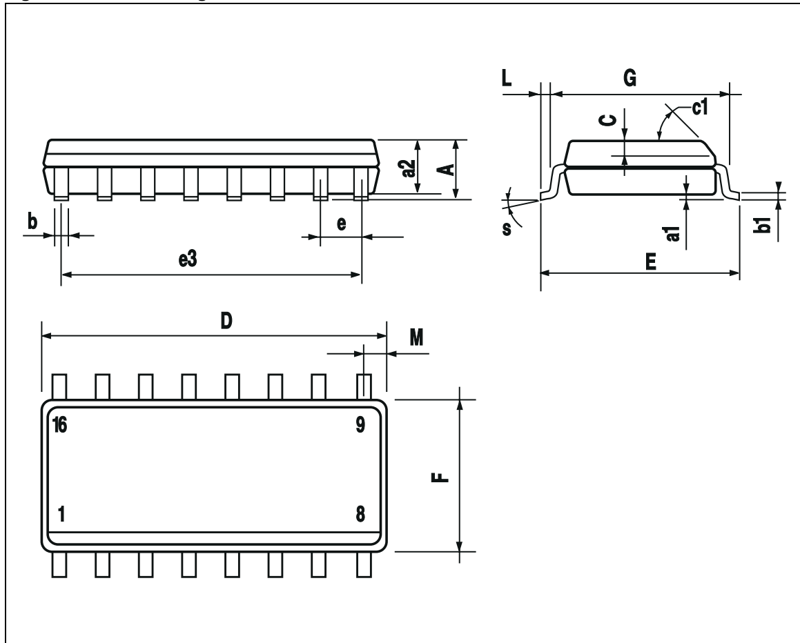
Figure 32. SO-16 Package Dimensions
