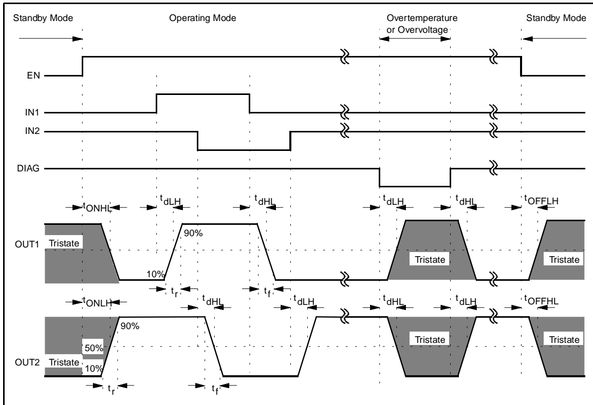
Figure 2. Timing Diagram.
