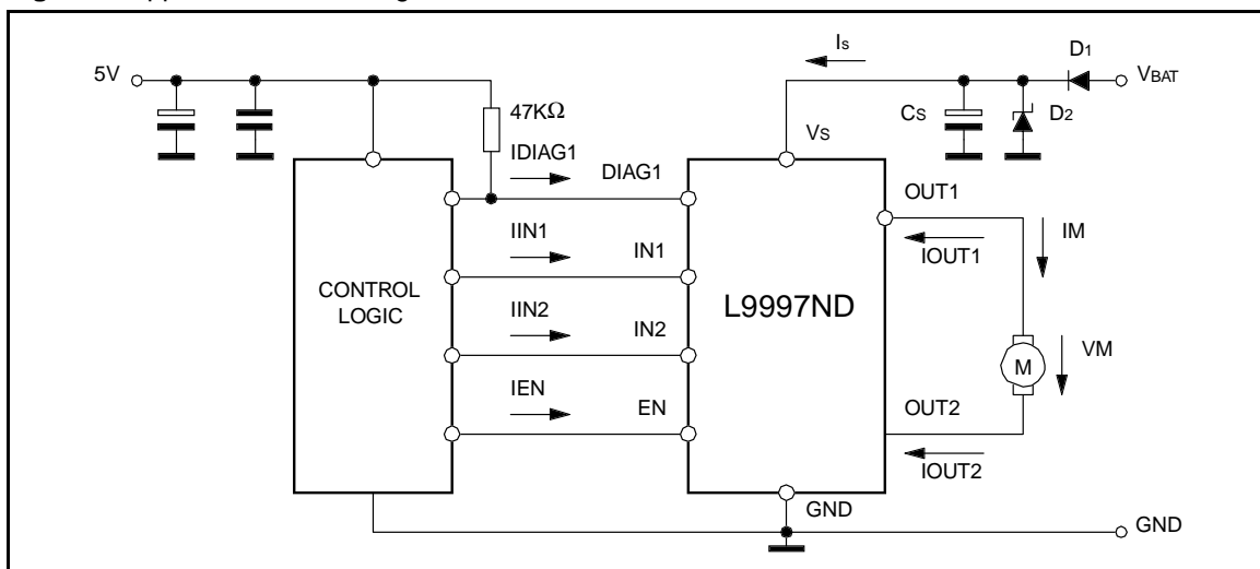
Figure 1: Application Circuit Diagram.
