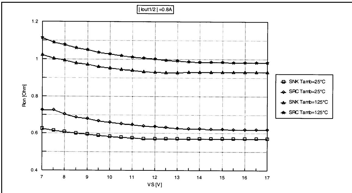
Figure 5. ON-Resistance versus supply voltage.
