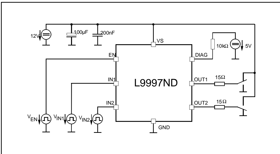
Figure 7. Test circuit.
