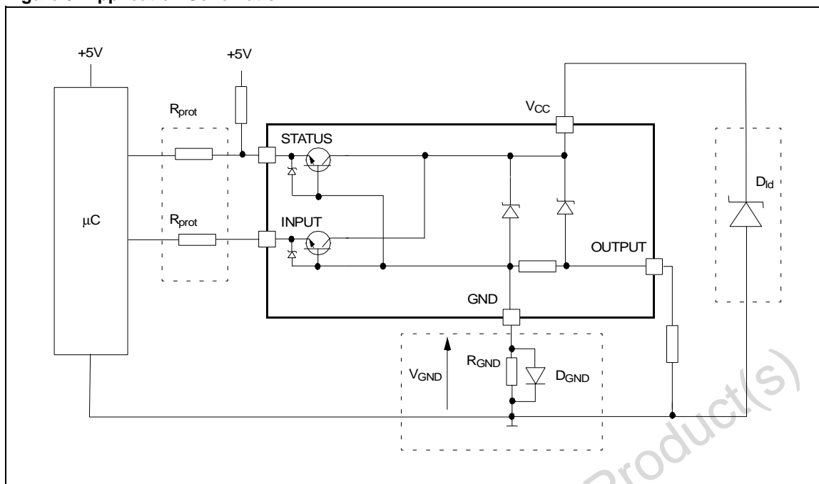
Figure 8. Application Schematic
