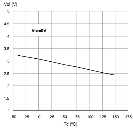
Figure 20. Openload Off State Voltage Detection Threshold
