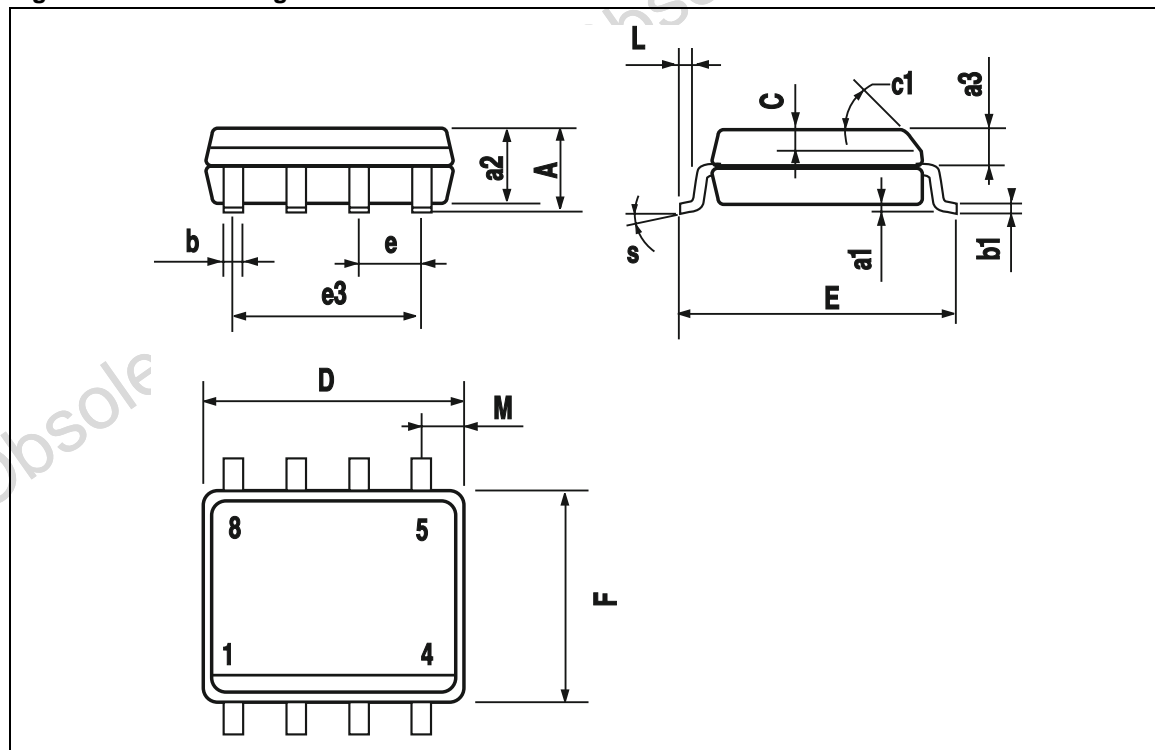
Figure 32. SO-8 Package Dimensions
