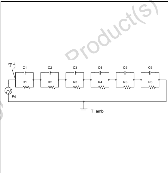
Figure 31. Thermal fitting model of a single channel HSD in SO-8
