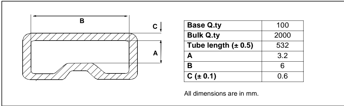
Figure 33. SO-8 TUBE SHIPMENT (no suffix)
