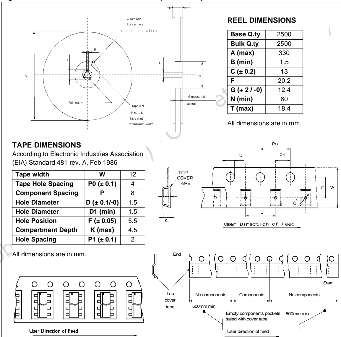
Figure 34. SO-8 TAPE AND REEL SHIPMENT (suffix "TR")
