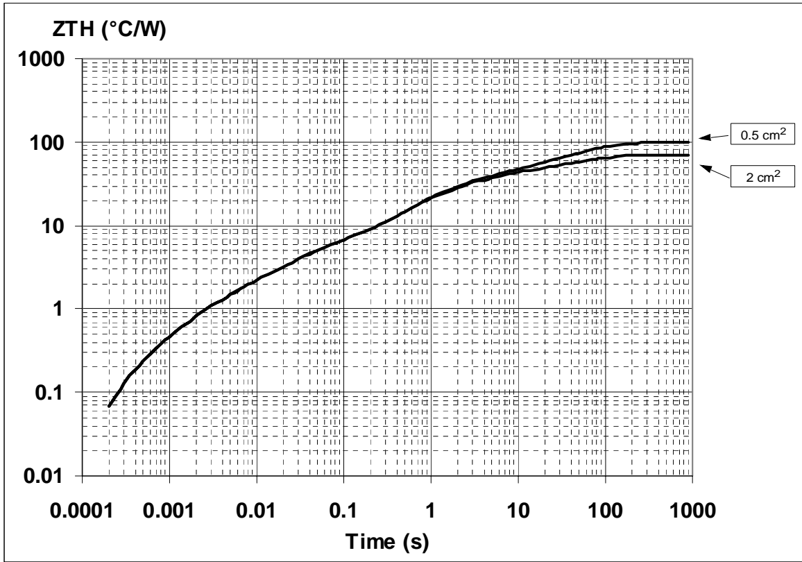
Figure 30. SO-8 Thermal Impedance Junction Ambient Single Pulse
