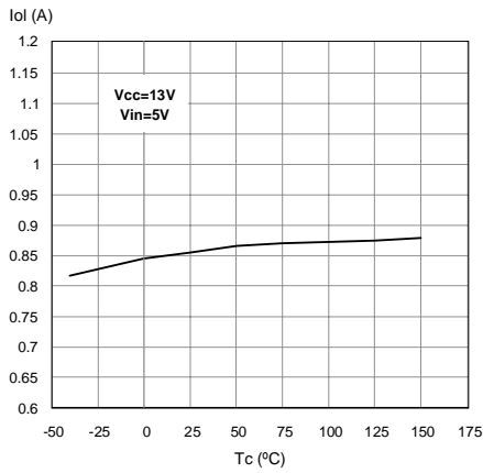
Figure 18. Openload On State Detection Threshold
