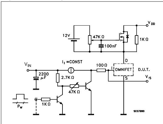
Fig. 5: Input Charge Test Circuit
