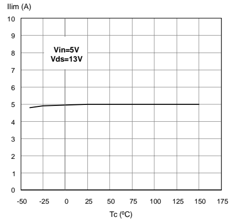
Normalized Current Limit Vs. Junction Temperature
