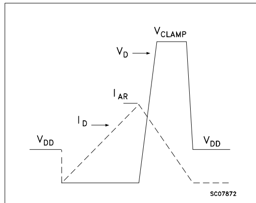
Fig. 4: Unclamped Inductive Waveforms
