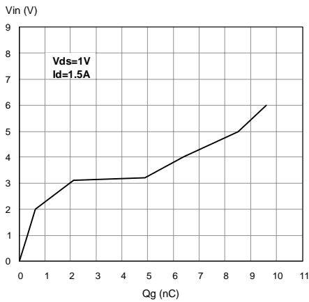
Input Voltage Vs. Input Charge
