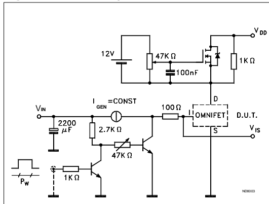
Figure 5: Input Charge Test Circuit
