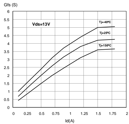
Transconductance
