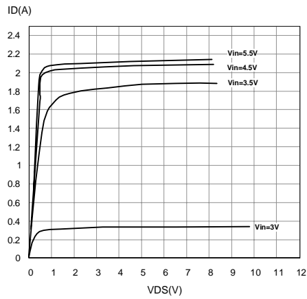
Output Characteristics
