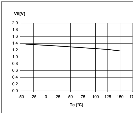
Figure 12. Input low-level voltage
