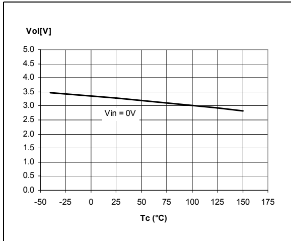
Figure 22. Turn-off voltage slope
