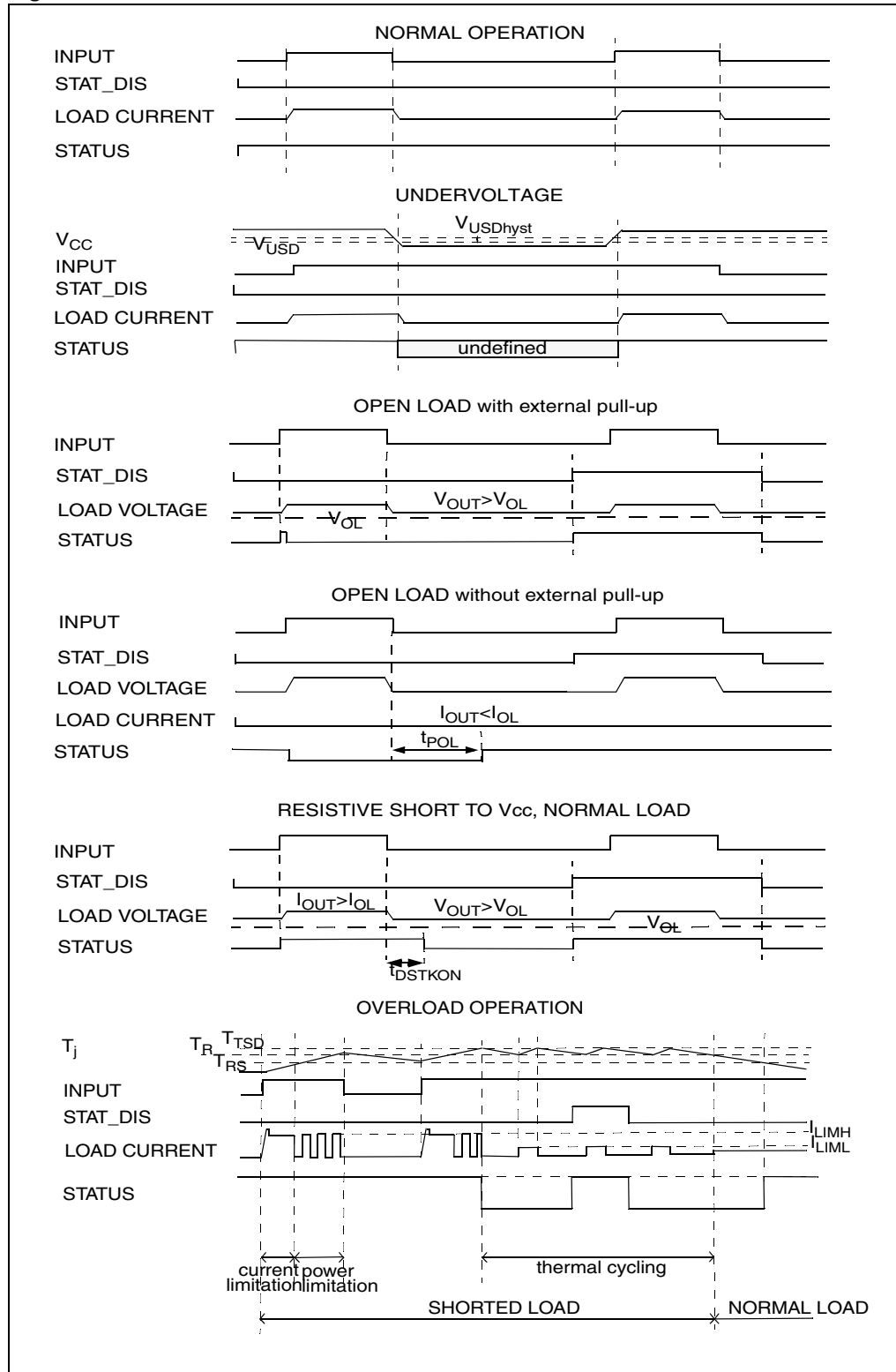
Figure 7. Waveforms
