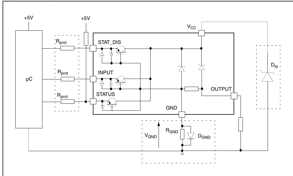
Figure 28. Application schematic
