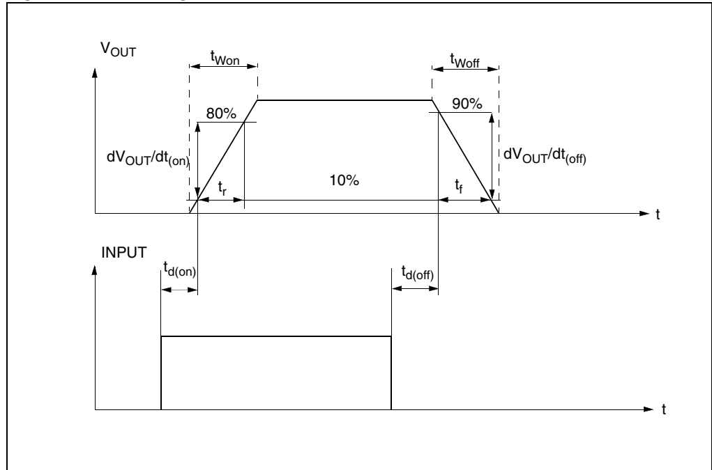
Figure 6. Switching characteristics
