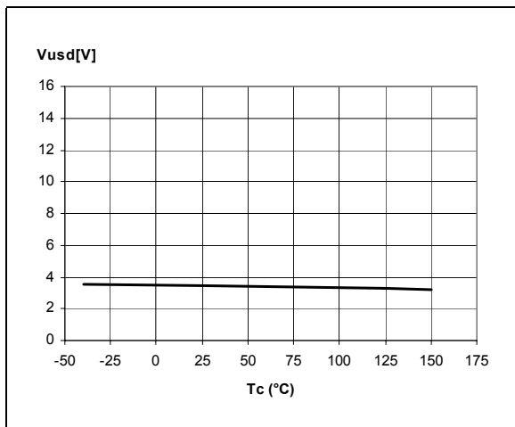
Figure 24. Undervoltage shutdown
