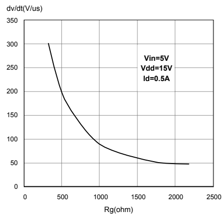
Figure 20. Turn-off drain source voltage slope (part 1/2)
