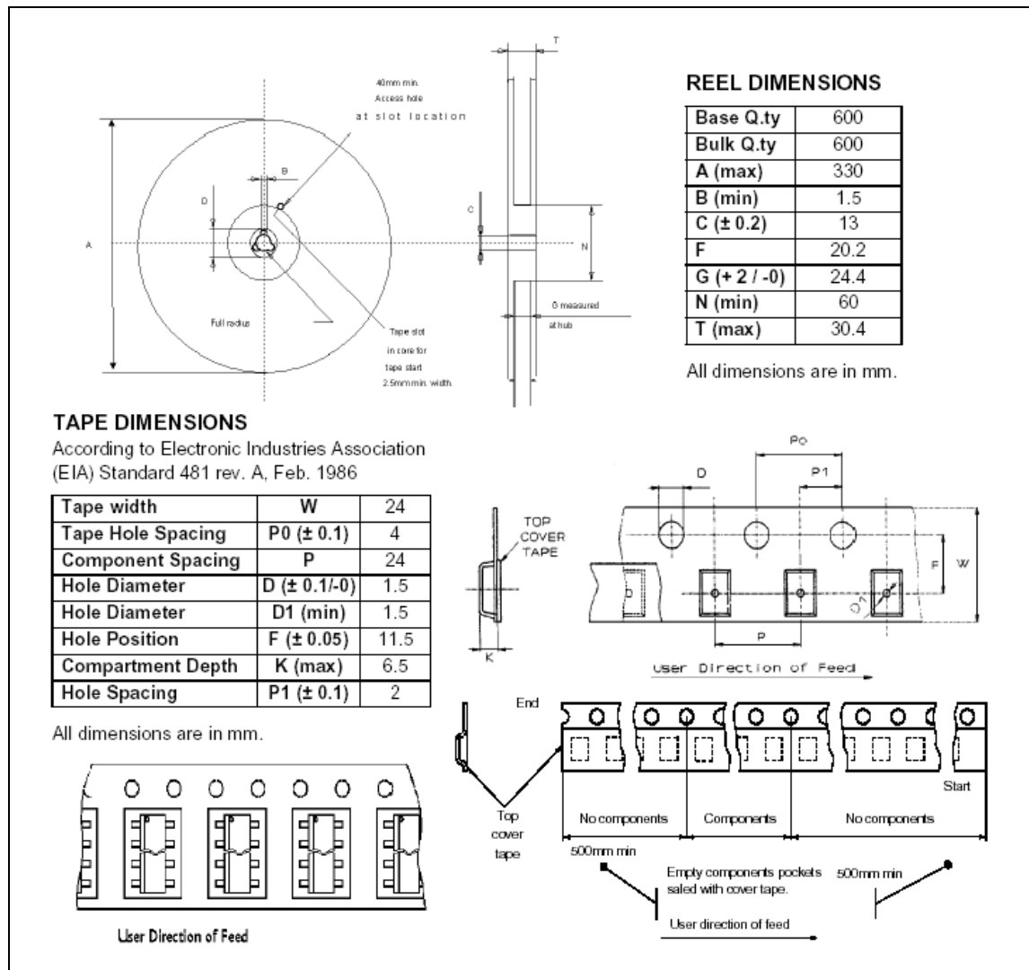
Figure 11. Tape and Reel Shipment (Suffix “TR”)
