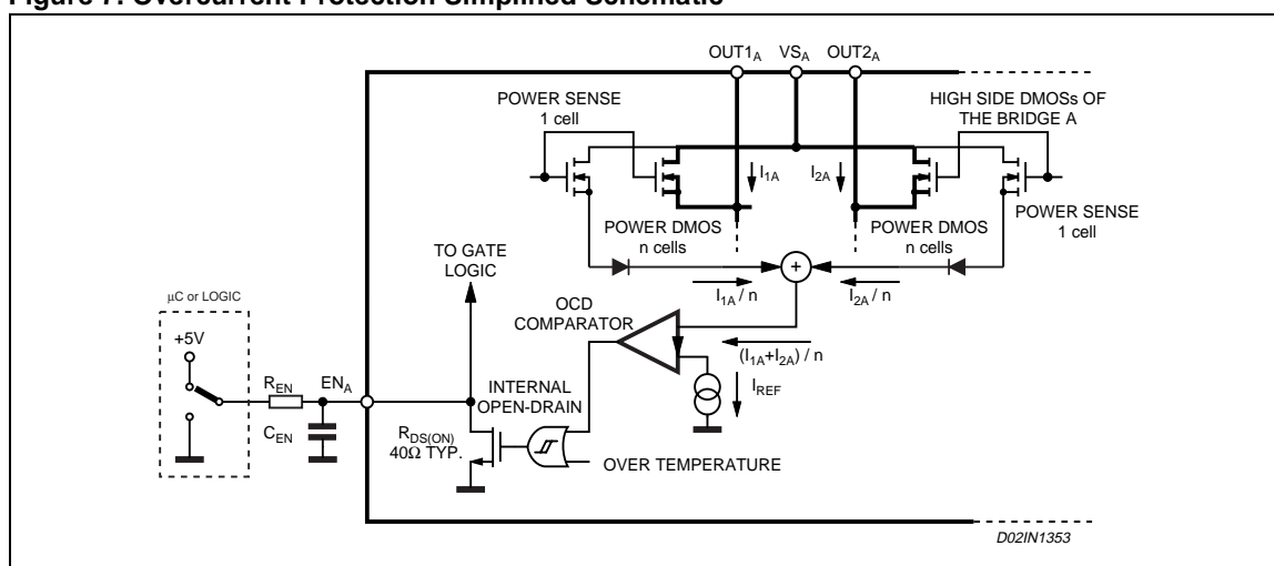
Figure 7. Overcurrent Protection Simplified Schematic
