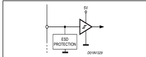
Figure 4. Logic Inputs Internal Structure
