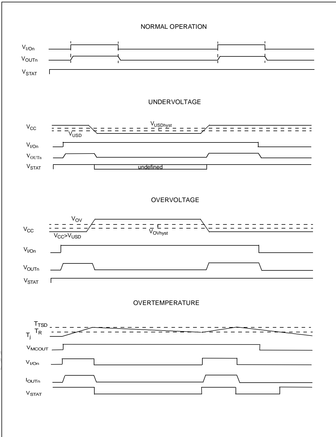
Figure 1: Waveforms
