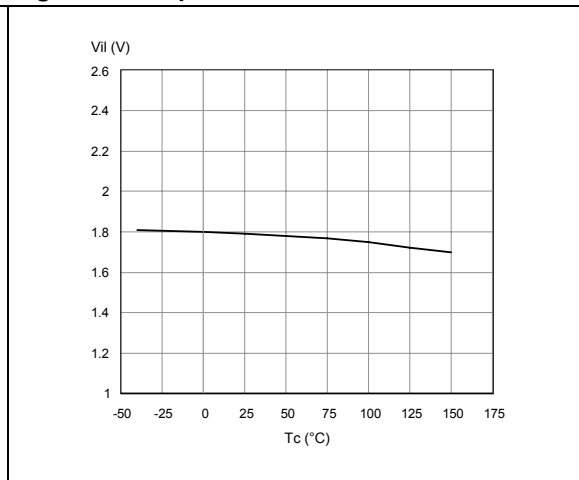
Figure 18. Input low-level
