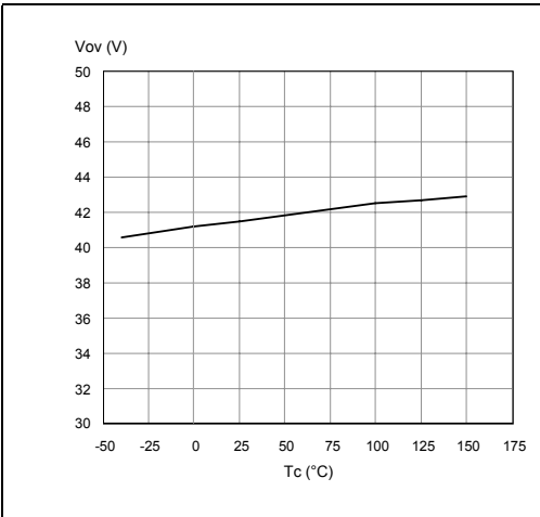
Figure 11. Over-voltage shutdown
